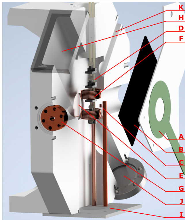
Fig. 2. Exploded view of the experimental measurement chamber. The following parts are shown: (a) PCB shimming coil, (b) \beta -detectors, (c) ^1\text{H} magnetometer, (d) sample ladder, (e) \beta -windows, (f) rf-excitation coil, (g) collimator, (h) front viewport, (i) bottom plate with viewport, and feedthroughs, and two empty flanges for expansion purposes (j, k). See text for further details.
