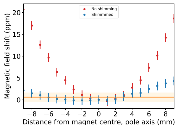
Fig. 5. Spatial deviation of the magnetic field when going away from the magnet's center towards its poles. Red symbols: shimming coils turned off; Blue symbols: shimming coils on; Orange line shows the median field across the sample site and the shade area indicates a 1 ppm difference from this line. (For interpretation of the references to color in this figure legend, the reader is referred to the web version of this article.)
