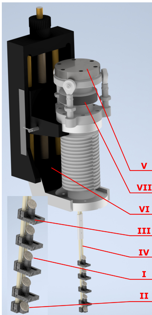
Fig. 3. Sample exchange ladder that allows for the rapid exchange of samples. Shown are (i) the mica sheet sample holder, (ii) reference crystals, (iii) PLA mounting structures, (iv) ceramic rods, (v) vacuum flange, (vi) the linear translation stage and (vii) tilt adjust.
