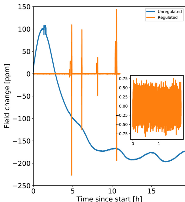
Fig. 4. The change of the magnetic field compared to a reference value over time with the locking system off (blue) and on (orange). The inset shows a zoom of the regulated data. The spikes in the data are due to interventions on the experimental chamber requiring the regulation to be temporarily turned off. Once turned back on, the system cycles through most of its range before regaining the locked frequency. The initial drift of the unregulated data is due to slow equilibration of the magnet and power supply. The subsequent oscillations are caused by fluctuations in the cooling water and ambient temperature. (For interpretation of the references to color in this figure legend, the reader is referred to the web version of this article.)
