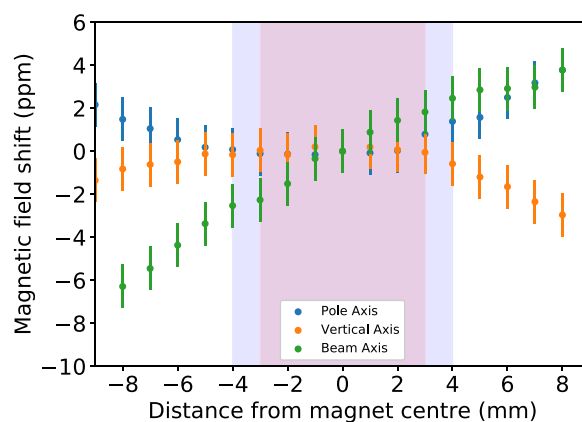
Fig. 6. Final shimming results for the magnetic field along all three axes, relative to the magnetic field in the center of the magnet (taken as 0 ppm). Blue symbols: field deviation along the central pole-to-pole axis, orange symbols: deviation along the vertical axis, green symbols: deviation in the horizontal (beam) direction. The shaded blue area indicates the sample space in the pole-to-pole direction, and the shaded red area the sample space in the other two directions. (For interpretation of the references to color in this figure legend, the reader is referred to the web version of this article.)
