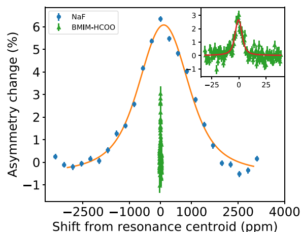
Fig. 7. A comparison between the resonance width of ^{26}\text{Na} in a solid state host (NaF; blue), and a liquid state host (BMIM-HCOO; green). The deviation from the center of each peak is given on the x-axis. The inset shows the resonance in the liquid host. (For interpretation of the references to color in this figure legend, the reader is referred to the web version of this article.)
