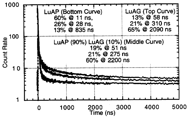
Figure 6: X-ray excited decay time spectra of cerium doped LuAP, LuAG, and 90% LuAP contaminated with 10% LuAG.
