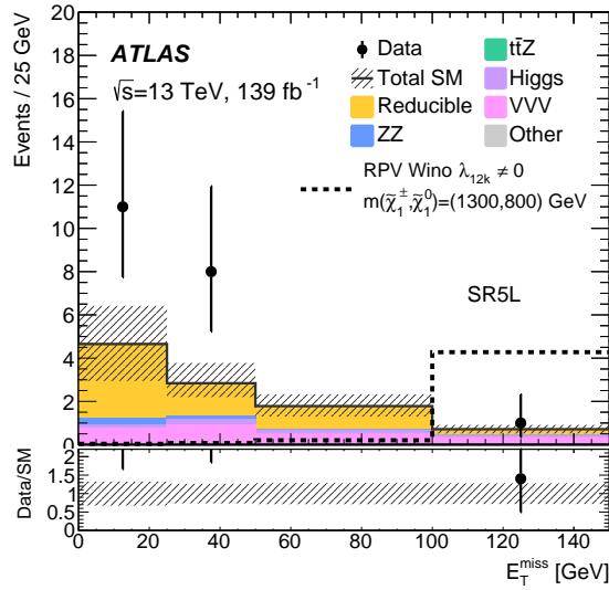
Figure 8: The E_T^{\text{miss}} distribution in (a) SR0-ZZ loose and SR0-ZZ tight , (b) SR0-ZZ loose bveto and SR0-ZZ tight bveto , and (c) SR5L for events passing the signal region requirements except the E_T^{\text{miss}} requirement. Distributions for data, the estimated SM backgrounds after the background-only fit, and an example SUSY scenario are shown. “Other” is the sum of the tWZ , t\bar{t}WW , t\bar{t}ZZ , t\bar{t}WH , t\bar{t}HH , t\bar{t}tW , and t\bar{t}t\bar{t} backgrounds. The last bin captures the overflow events. The lower panel shows the ratio of the observed data to the expected SM background yield in each bin. Both the statistical and systematic uncertainties in the SM background are included in the shaded band. The red arrows indicate the E_T^{\text{miss}} selections in the signal regions.
