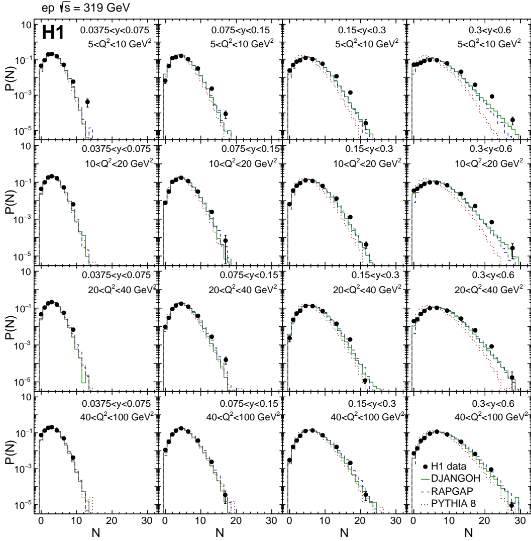
Figure 2: Charged particle multiplicity distributions P(N) as a function of the number of particles N at \sqrt{s} = 319 \text{ GeV} ep collisions. Different panels correspond to different Q^2 and y bins, as indicated by the text in the figure. The phase space restrictions are given in Table 1. Predictions from DJANGO, RAPGAP and PYTHIA 8 are also shown. The total uncertainty is denoted by the error bars.
