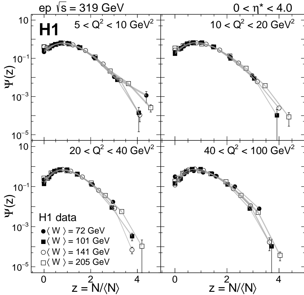
Figure 10: KNO function \Psi(z) as a function of z measured at \sqrt{s} = 319 GeV in ep collisions in bins of Q^2 with an additional restriction to the current hemisphere 0 < \eta^* < 4 . Further phase space restrictions are given in Table 1. The total uncertainty is denoted by the error bars.
