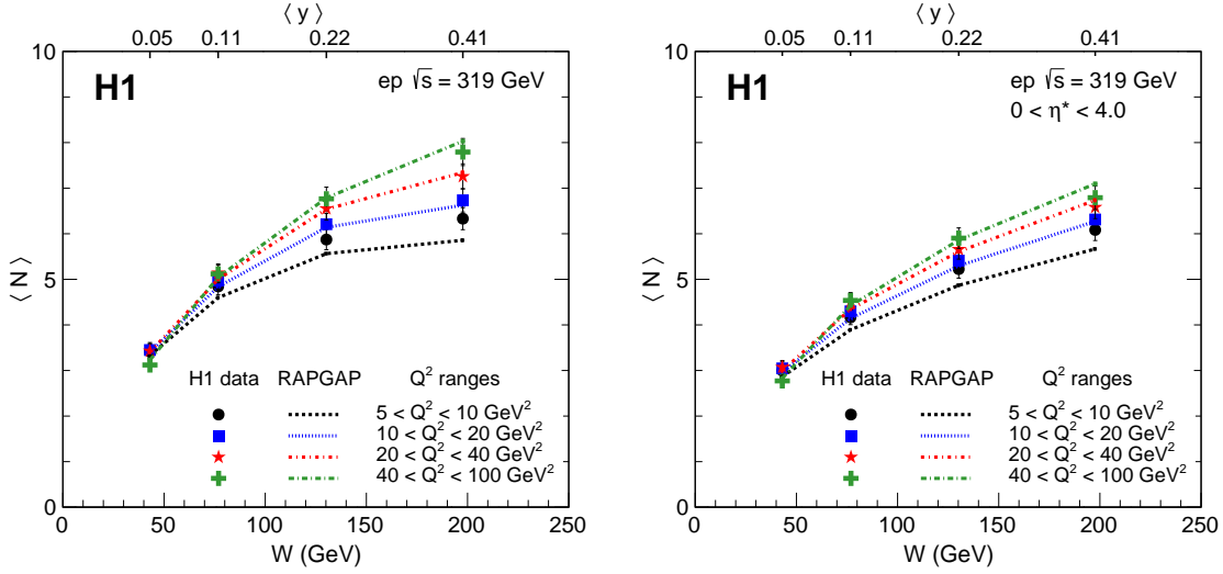
Figure 8: Mean multiplicity \langle N \rangle as a function of W measured at \sqrt{s} = 319 \text{ GeV} ep collisions (left) and with an additional restriction to the current hemisphere 0 < \eta^* < 4 (right). Further phase space restrictions are given in Table 1. The corresponding \langle y \rangle is indicated by the top axis for each measured W . Predictions from the RAPGAP model are shown by dashed lines. The total uncertainty is represented by the error bar.
