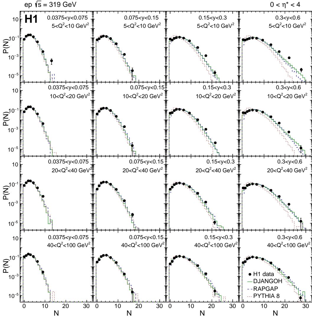
Figure 7: Charged particle multiplicity distributions P(N) as a function of the number of particles N at \sqrt{s} = 319 GeV ep collisions with additional restriction to the current hemisphere 0 < \eta^* < 4 . Further phase space restrictions are given in Table 1. Different panels correspond to different Q^2 and y bins, as indicated by the text in the figure. Predictions from DJANGO, RAPGAP and PYTHIA 8 are also shown. The total uncertainty is denoted by the error bars.
