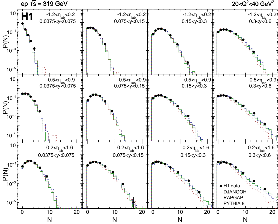
Figure 5: Charged particle multiplicity distributions P(N) as a function of the number of particles N at \sqrt{s} = 319 GeV ep collisions in the range 20 < Q^2 < 40 GeV 2 . Further phase space restrictions are given in Table 1. Different panels correspond to different \eta_{\text{lab}} and y bins, as indicated by the text in the figure. Predictions from DJANGO, RAPGAP and PYTHIA 8 are also shown. The total uncertainty is denoted by the error bars.
