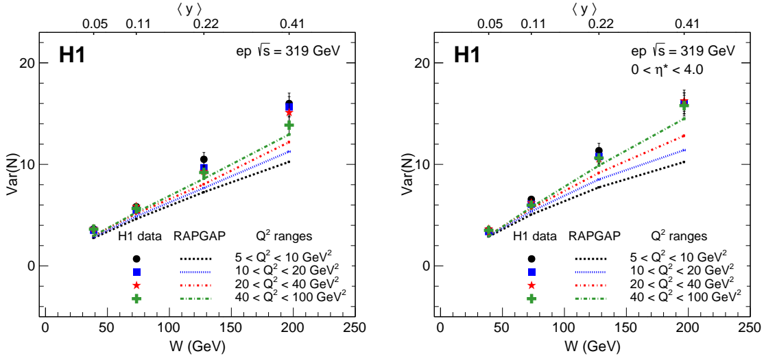
Figure 9: Second moment (variance) of the multiplicity distributions Var(N) as a function of W measured at \sqrt{s} = 319 \text{ GeV} ep collisions (left) and with an additional restriction to the current hemisphere 0 < \eta^* < 4 (right). Further phase space restrictions are given in Table 1. The corresponding \langle y \rangle is indicated by the top axis for each measured W . Predictions from the RAPGAP model are shown by dashed lines. The total uncertainty is represented by the error bar.
