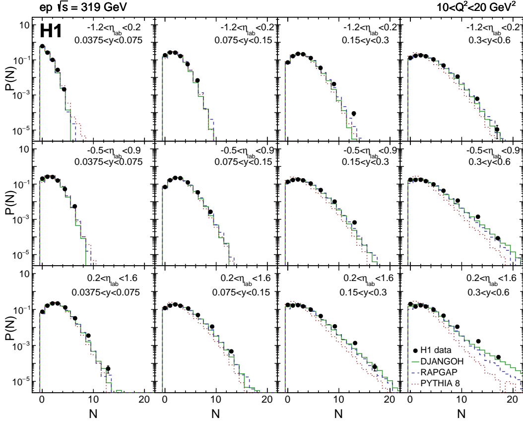
Figure 4: Charged particle multiplicity distributions P(N) as a function of the number of particles N at \sqrt{s} = 319 GeV ep collisions in the range 10 < Q^2 < 20 GeV 2 . Further phase space restrictions are given in Table 1. Different panels correspond to different \eta_{\text{lab}} and y bins, as indicated by the text in the figure. Predictions from DJANGO, RAPGAP and PYTHIA 8 are also shown. The total uncertainty is denoted by the error bars.
