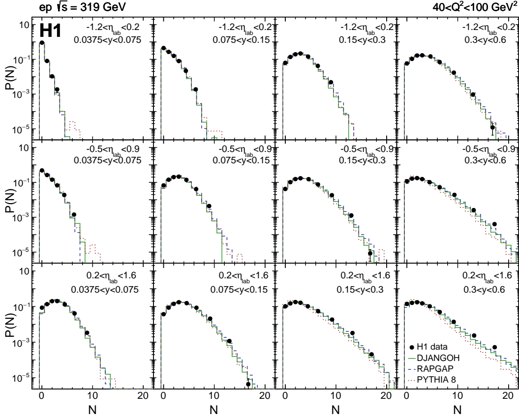
Figure 6: Charged particle multiplicity distributions P(N) as a function of the number of particles N at \sqrt{s} = 319 GeV ep collisions in the range 40 < Q^2 < 100 GeV 2 . Further phase space restrictions are given in Table 1. Different panels correspond to different \eta_{\text{lab}} and y bins, as indicated by the text in the figure. Predictions from DJANGO, RAPGAP and PYTHIA 8 are also shown. The total uncertainty is denoted by the error bars.
