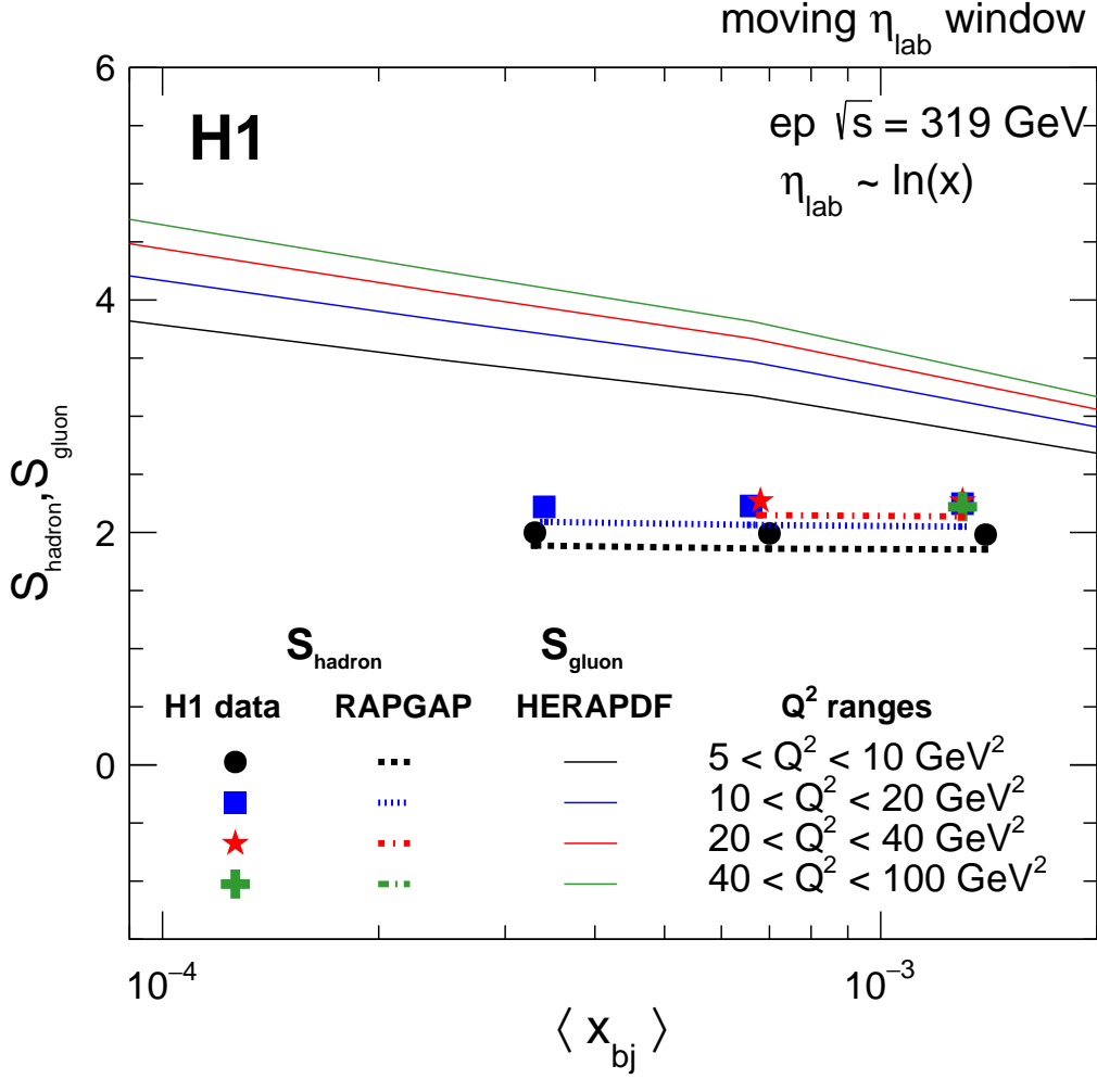
Figure 11: Hadron entropy S_{\text{hadron}} derived from multiplicity distributions, reported as a function of \langle x_{bj} \rangle in different Q^2 ranges, measured in \sqrt{s} = 319 \text{ GeV} ep collisions. For each \langle x_{bj} \rangle , the multiplicity is determined in a dedicated pseudorapidity window as discussed in the text. Further phase space restrictions are given in Table 1. Predictions for S_{\text{hadron}} from the RAPGAP model and for the entanglement entropy S_{\text{gluon}} based on an entanglement model are shown by the dashed lines and solid lines, respectively. For each Q^2 range, the value of the lower boundary is used for predicting S_{\text{gluon}} . The total uncertainty on the data is represented by the error bars.
