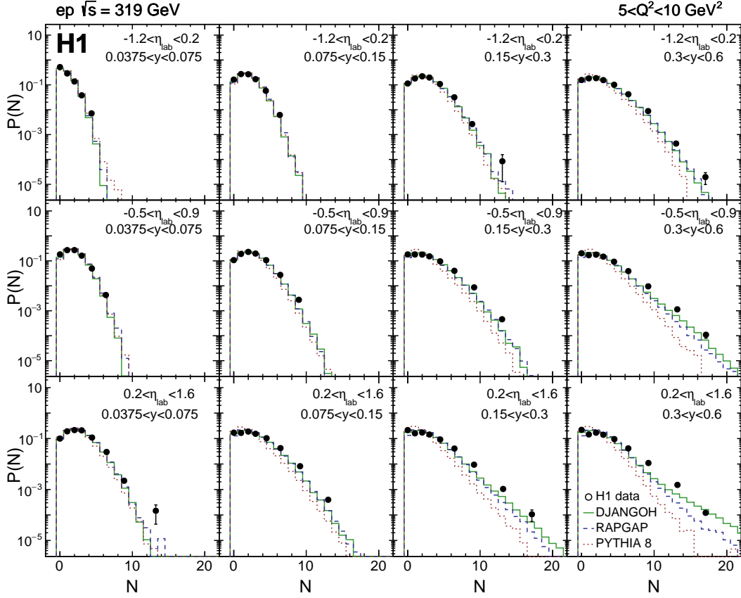
Figure 3: Charged particle multiplicity distributions P(N) as a function of the number of particles N at \sqrt{s} = 319 GeV ep collisions in the range 5 < Q^2 < 10 GeV 2 . Further phase space restrictions are given in Table 1. Different panels correspond to different \eta_{\text{lab}} and y bins, as indicated by the text in the figure. Predictions from DJANGO, RAPGAP and PYTHIA 8 are also shown. The total uncertainty is denoted by the error bars.
