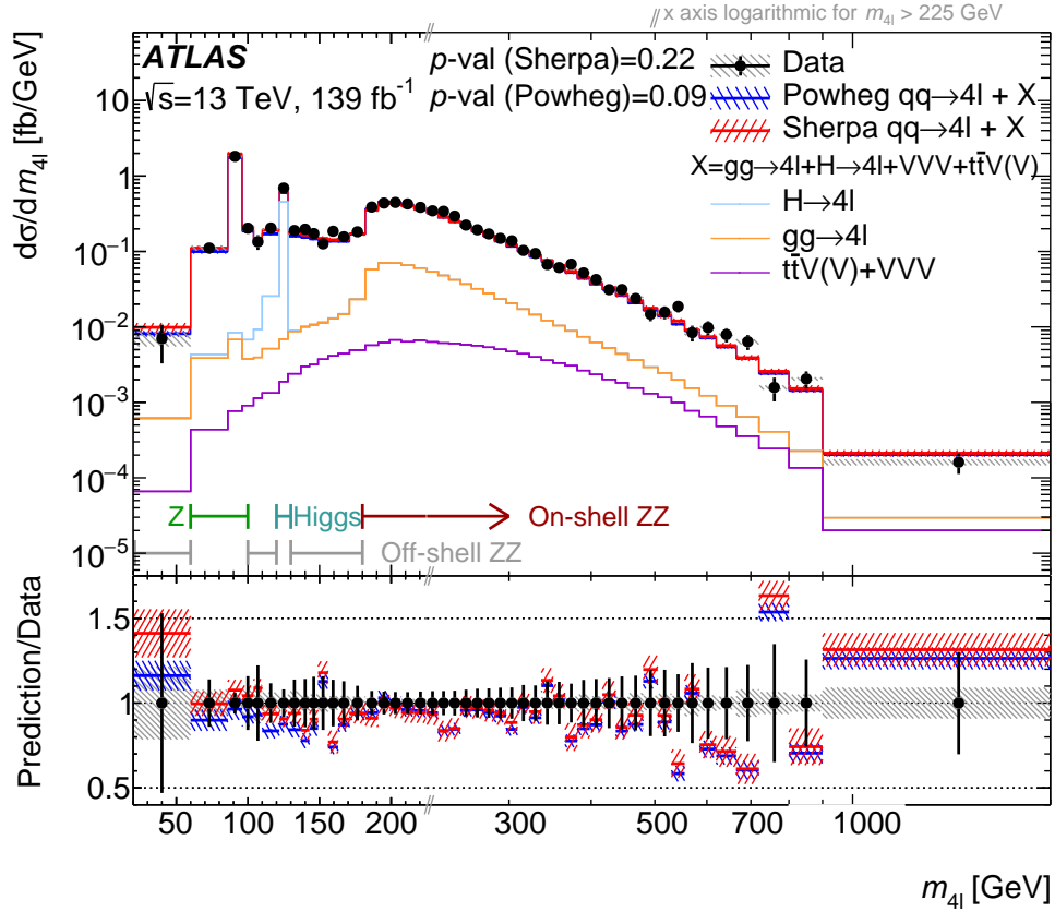
Figure 4: Differential cross-section as a function of m_{4\ell} . The measured data (black points) are compared with the SM prediction using either SHERPA (red, with red hashed band for the uncertainty) or POWHEG + PYTHIA8 (blue, with blue hashed band for the uncertainty) to model the q\bar{q} \rightarrow 4\ell contribution. The error bars on the data points give the total uncertainty and the grey hashed band gives the systematic uncertainty. The breakdown of the contribution from different SM processes is also shown in successive stacked histograms. The short vertical lines terminating horizontal lines indicate the boundaries of the different m_{4\ell} regions in which the other variables are measured. The p -value is the probability for the \chi^2 , with the number of degrees of freedom equal to the number of bins in the distribution, to have at least the observed value, given the SM prediction. The lower panel shows the ratio of the SM predictions to the data. The x -axis is on a linear scale until m_{4\ell} = 216 GeV, where it switches to a logarithmic scale.
