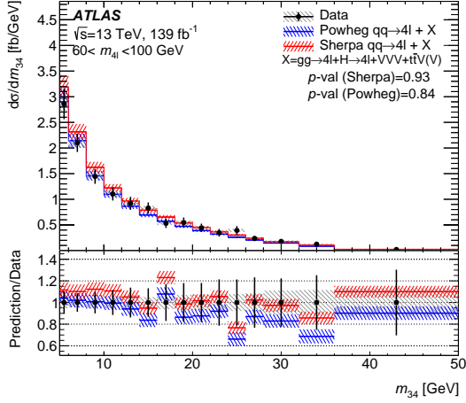
(a) Z \rightarrow 4\ell region
