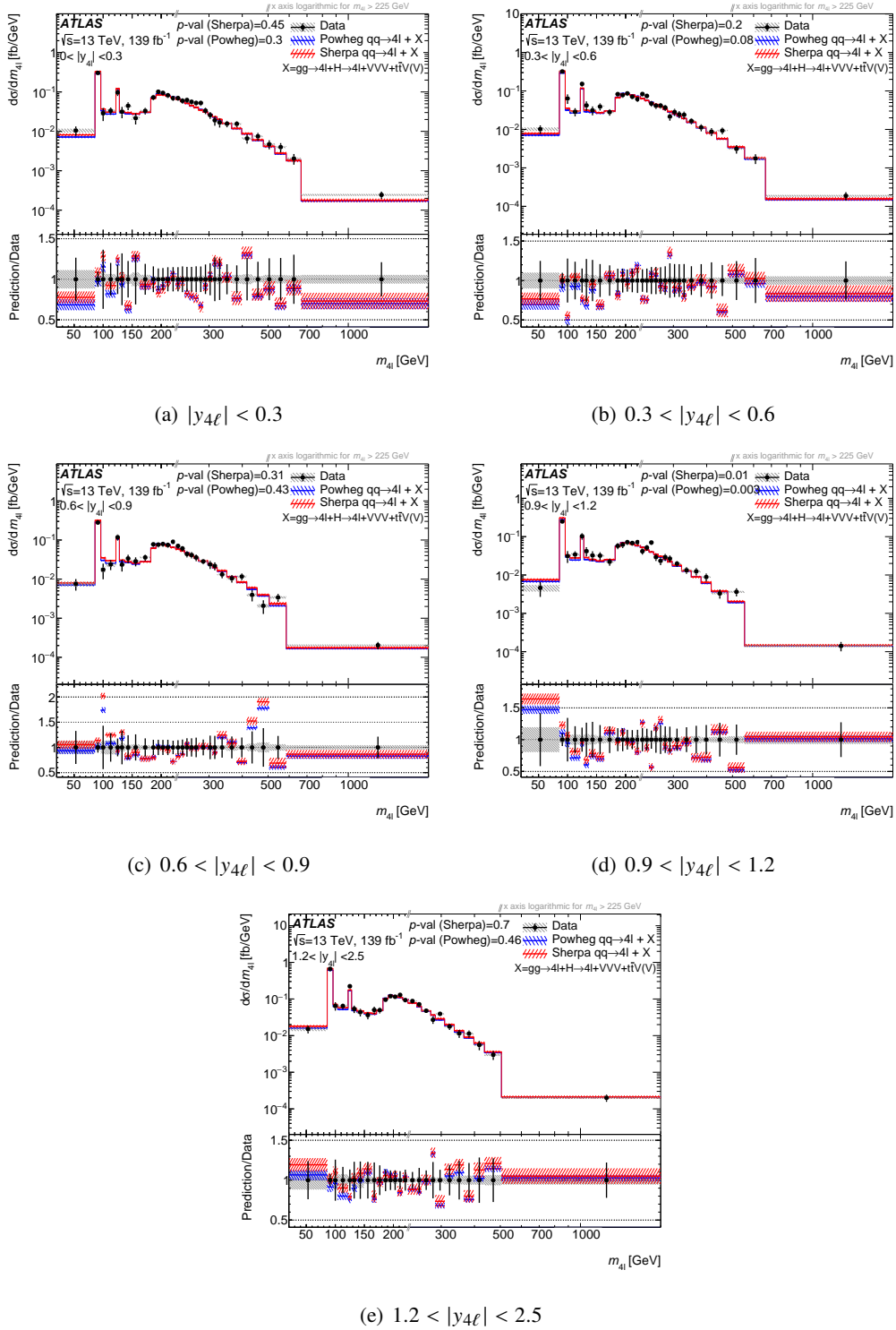
Figure 15: Differential cross-section as a function of m_{4\ell} in |y_{4\ell}| slices. The measured data (black points) are compared with the SM prediction using either SHERPA (red, with red hashed band for the uncertainty) or POWHEG + PYTHIA8 (blue, with blue hashed band for the uncertainty) to model the q\bar{q} \rightarrow 4\ell contribution. The error bars on the data points give the total uncertainty and the grey hashed band gives the systematic uncertainty. The p -value is the probability for the \chi^2 , with the number of degrees of freedom equal to the number of bins in the distribution, to have at least the observed value, given the SM prediction. The lower panel shows the ratio of the SM predictions to the data. The x -axis is on a linear scale until m_{4\ell} = 216 GeV, where it switches to a logarithmic scale.
