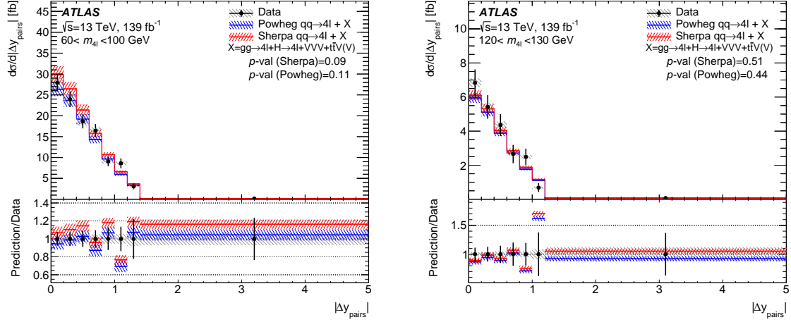
(a) Z \rightarrow 4\ell region
