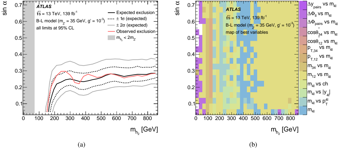
Figure 12: (a) Exclusion contour at 95% confidence level for the B-L gauge model [102] in the plane of \sin \alpha versus m_{h_2} for m_{Z'} = 35 GeV and g' = 10^{-3} . The red line shows the observed exclusion and the solid black line shows the expected exclusion, with the dashed black lines indicating the \pm 1\sigma and \pm 2\sigma uncertainty bands. The region above and to the left of the lines is excluded, up to the grey band, which shows the region m_{h_2} < 2m_{Z'} , where the four-lepton final state has no sensitivity. (b) Colour palette indicating which observable has the highest expected sensitivity at each point in the parameter space and is used to set the limit.
