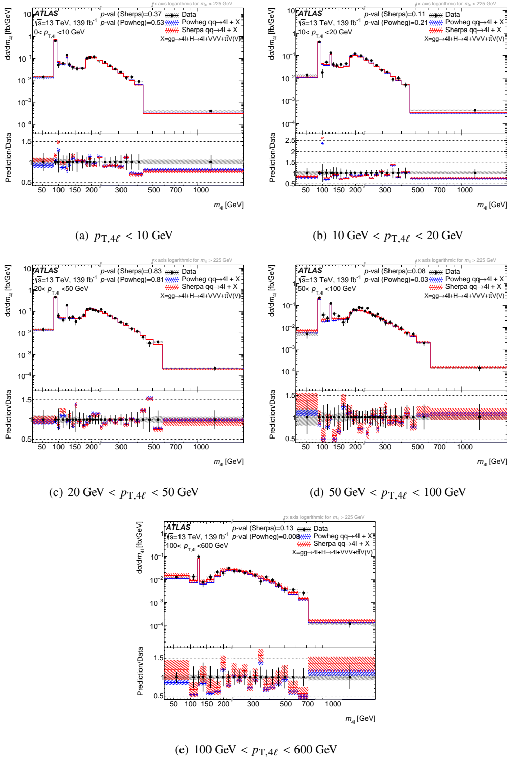
Figure 14: Differential cross-section as a function of m_{4\ell} in p_{T,4\ell} slices. The measured data (black points) are compared with the SM prediction using either SHERPA (red, with red hashed band for the uncertainty) or POWHEG + PYTHIA8 (blue, with blue hashed band for the uncertainty) to model the q\bar{q} \rightarrow 4\ell contribution. The error bars on the data points give the total uncertainty and the grey hashed band gives the systematic uncertainty. The p -value is the probability for the \chi^2 , with the number of degrees of freedom equal to the number of bins in the distribution, to have at least the observed value, given the SM prediction. The lower panel shows the ratio of the SM predictions to the data. The x -axis is on a linear scale until m_{4\ell} = 216 GeV, where it switches to a logarithmic scale.
