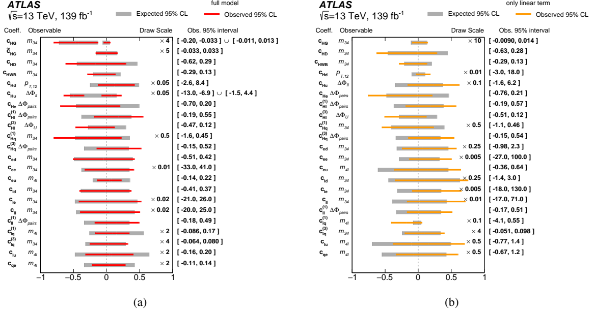
Figure 11: The expected and observed confidence intervals at 95% CL for the SMEFT Wilson coefficients, which are in units of \text{TeV}^{-2} , for (a) the full model and (b) only the linear terms. The multiplicative number shown to the right of plotted points indicates a scaling factor that is applied to the limit for the purpose of the plot, in order to show all coefficients on the same scale. The most sensitive observable indicated for each coefficient is used for the constraints. Only one coefficient is fitted at a time, with all others set to zero.
