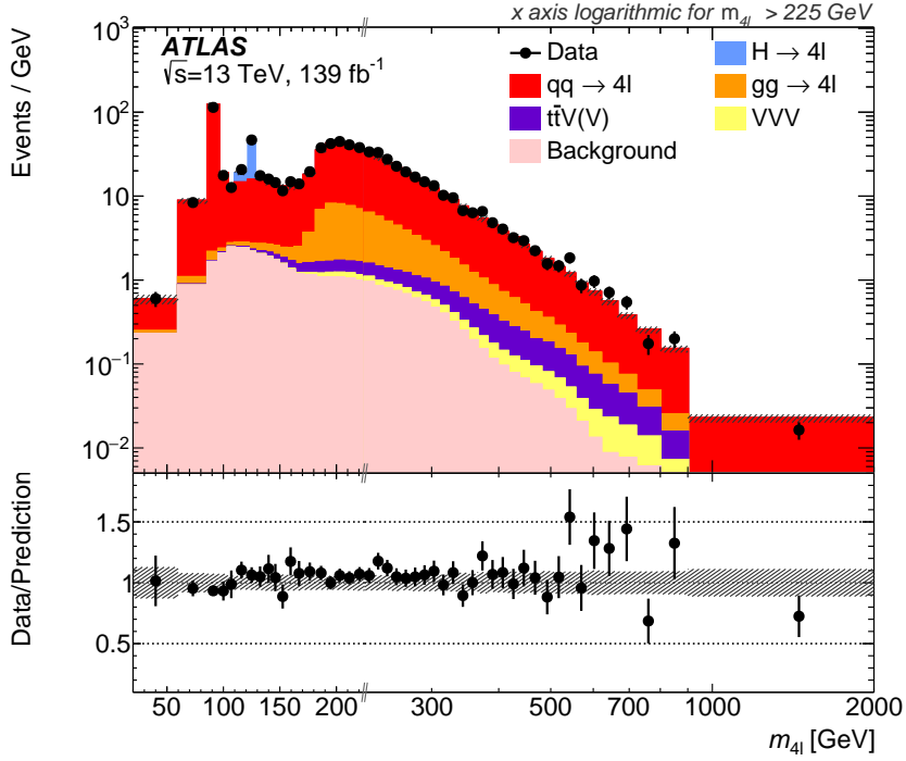
Figure 2: Observed reconstruction-level m_{4\ell} distribution compared with the SM prediction, using SHERPA for the q\bar{q} \rightarrow 4\ell simulation. The statistical uncertainty of the data is displayed as error bars and systematic uncertainties in the prediction are shown as a grey hashed band. The ratio of the data to the prediction is shown in the lower panel. The x -axis is on a linear scale until m_{4\ell} = 216 GeV, where it switches to a logarithmic scale, as indicated by the double dashes on the axis. There is one additional data event reconstructed with m_{4\ell} = 2.14 TeV, while 0.4 are expected from simulation for m_{4\ell} > 2 TeV.
