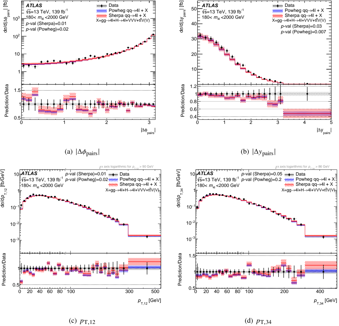
Figure 7: Differential cross-sections as a function of (a) |\Delta\phi_{\text{pairs}}| , (b) |\Delta y_{\text{pairs}}| , (c) p_{T,12} , and (d) p_{T,34} in the on-shell ZZ region. The measured data (black points) are compared with the SM prediction using either SHERPA (red, with red hashed band for the uncertainty) or POWHEG + PYTHIA8 (blue, with blue hashed band for the uncertainty) to model the q\bar{q} \rightarrow 4\ell contribution. The error bars on the data points give the total uncertainty and the grey hashed band gives the systematic uncertainty. The p -value is the probability for the \chi^2 , with the number of degrees of freedom equal to the number of bins in the distribution, to have at least the observed value, given the SM prediction. The lower panel shows the ratio of the SM predictions to the data. In (c) the x -axis is on a linear scale until p_{T,12} = 90 GeV, where it switches to a logarithmic scale; in (d) it switches at p_{T,34} = 86 GeV.
