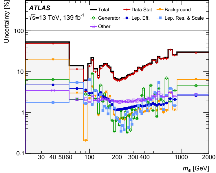
Figure 3: Uncertainty breakdown of the measured cross-section as a function of m_{4\ell} . “Lep. Eff.” refers to the uncertainties in the lepton efficiencies, “Lep. Res. & Scale” refers to the uncertainties in the lepton resolutions and scales, and the theory uncertainties are included in the “Generator” uncertainty. Contributions from the Monte Carlo statistical uncertainty and uncertainties in the luminosity and the inelastic cross-section are included in “Other”.
