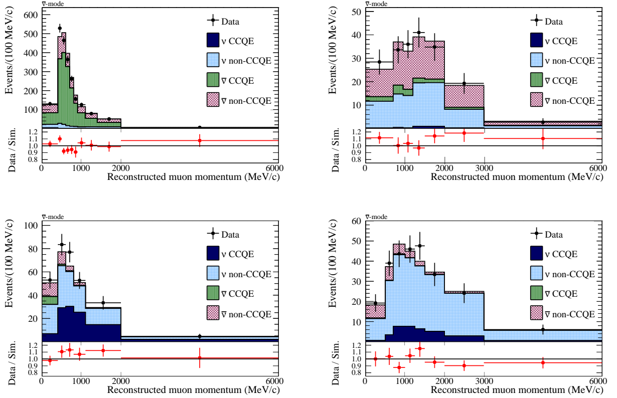
FIG. 13: Final state muon momentum distributions for the RHC \bar{\nu}_\mu (top) and \nu_\mu (bottom) CC 1-track (left) and CC N-track (right) FGD1 simulation samples. These distributions are before the ND280 fit.
