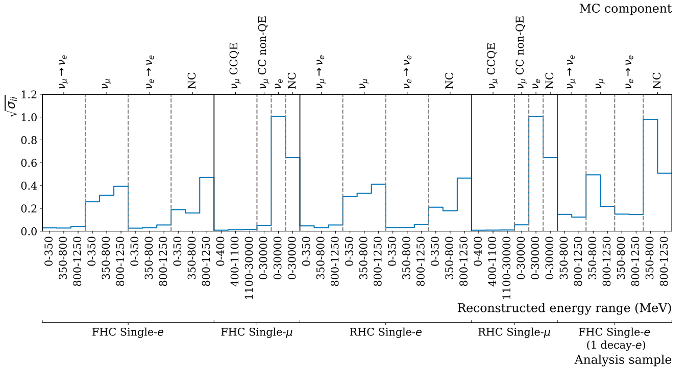
FIG. 33: Square root of the diagonal elements of the covariance matrix describing the systematic uncertainty associated to the modeling of the SK detector.
