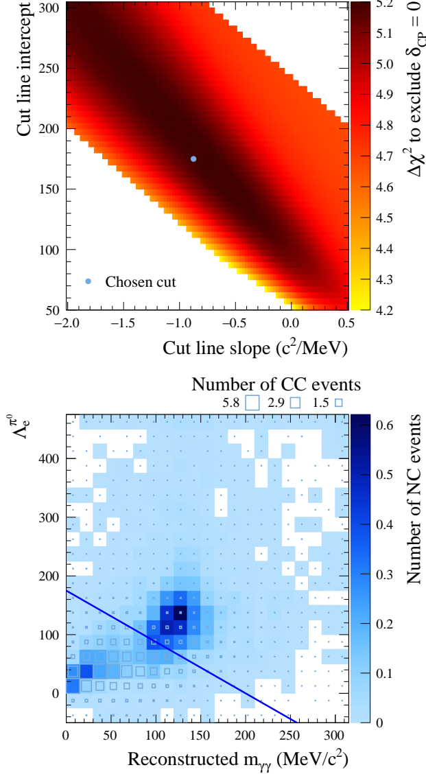
FIG. 29: The sensitivity to exclude \delta_{\text{CP}} = 0 as a function of the slope and intercept of the \text{NC}\pi^0 rejection cut line is shown on the top and the distribution of signal and background events is shown on the bottom, along with the line below which e -like events are selected.
