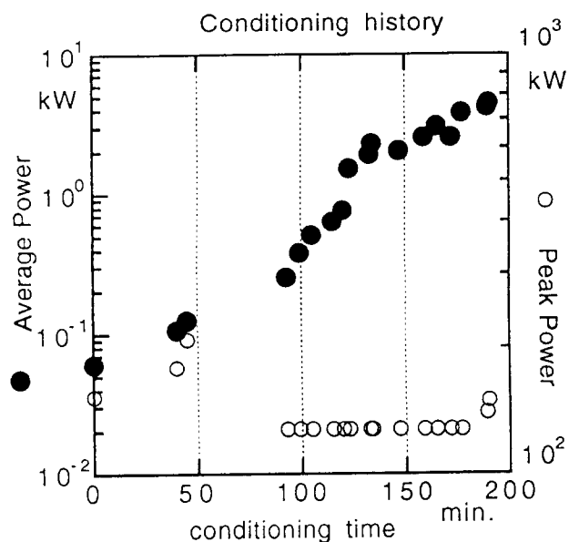
Fig. 8 Conditioning history of the DTL. The black & white circles show average and peak RF power, respectively.
