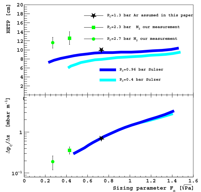
Fig. 6 Equivalent number of theoretical stages, HETP, and pressure drop per unit length, \Delta p_C/\Delta z vs. sizing parameter F_G . Blue (cyan) line: measurements with chlorobenzene/ethylbenzene mixtures at p_C = 0.96 \text{ bar} (0.40 bar), Sulzer CY Gauze Packing, partial data-set extracted from the Structured Packing brochure of Sulzer Ltd. website. The black stars correspond to the values assumed for the calculations of Aria distillation with argon in this paper, at p_C = 1.3 \text{ bar} . The full green dots (squares) correspond to the values measured during the nitrogen distillation Run A (Run B), at p_C = 2.7 \text{ bar} (2.3 bar), with the prototype column, discussed in Sect. 6, and are meant to be average values over the respective runs
