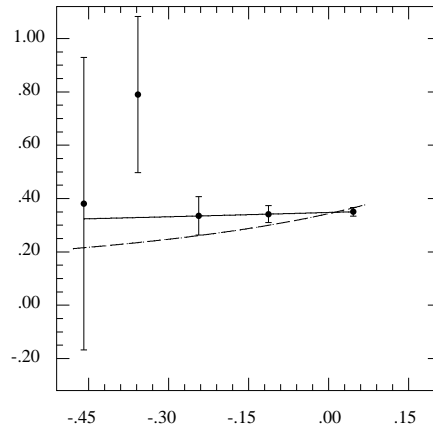
Figure 1. T_2(q^2) as a function of q^2 for K_H = .1330 . The curves show the pole dominance with either the lattice axial pole mass (dashed line) or with a free pole mass (full line).
