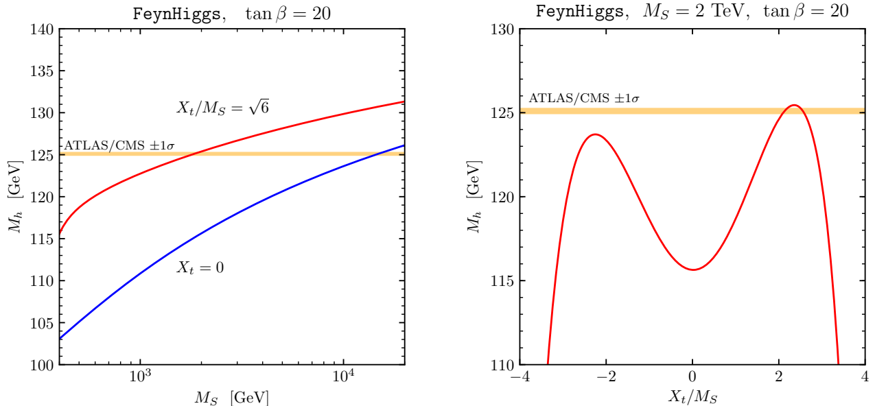
Figure 1: The lighter CP -even Higgs mass in the MSSM as a function of a common SUSY mass parameter M_S and of the stop mixing parameter X_t (normalized to M_S ). Both parameters are defined in the \overline{DR} scheme at the scale Q = M_S .
