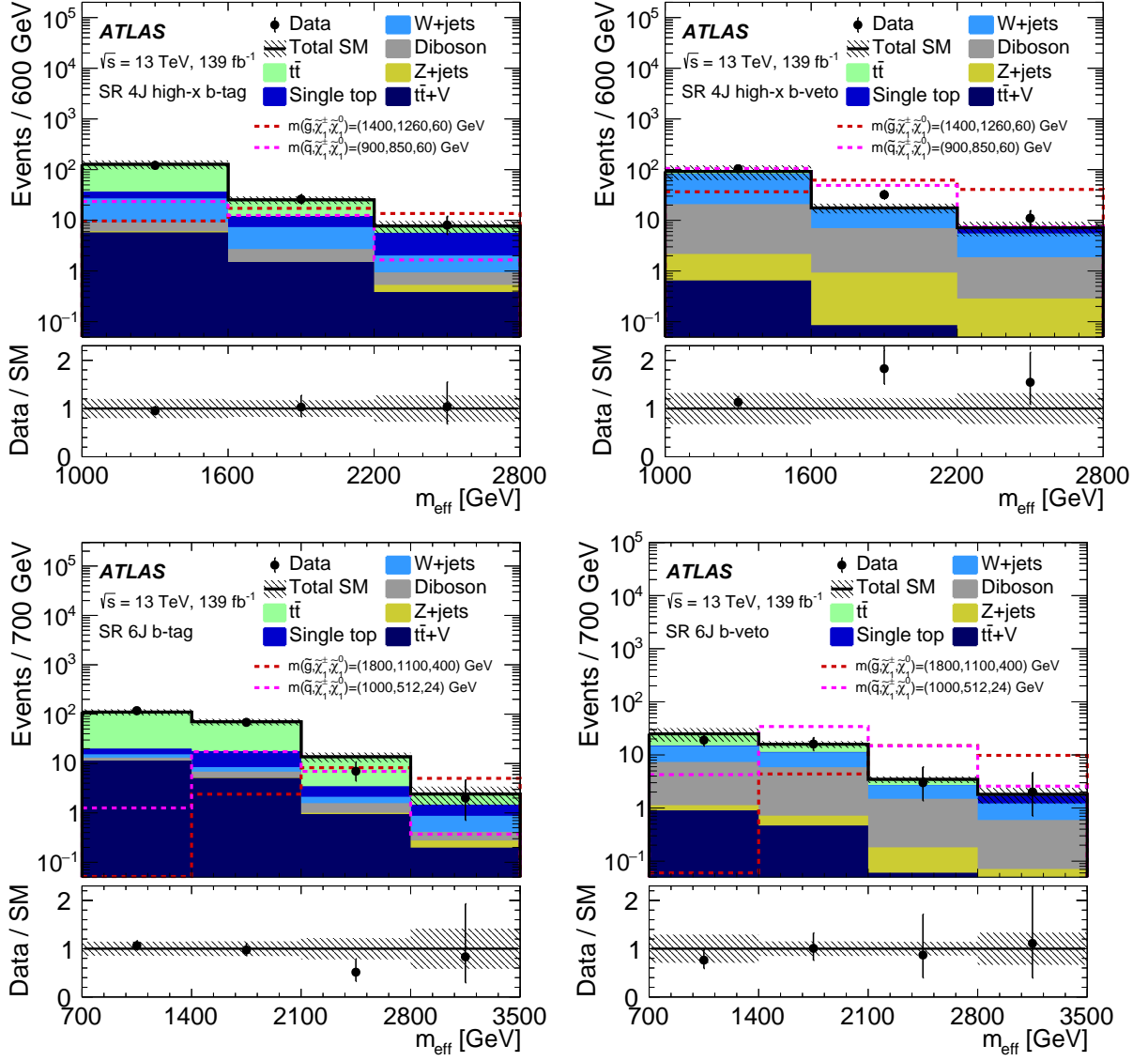
Figure 7: Post-fit m_{\text{eff}} distributions in the exclusion 4J high-x and 6J signal regions. The uncertainty bands include all statistical and systematic uncertainties. The dashed lines represent benchmark signal points. Overflow events are included in the last bin.
