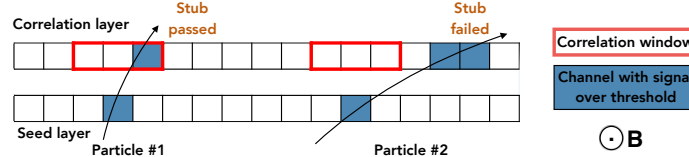
Figure 2: Illustration of the stub concept: particles generating a hit in the 'correlation layer' which is inside the 'correlation window' (indicated by red squares in the figure) will result in a stub being produced by the front-end chip's correlation logic.
