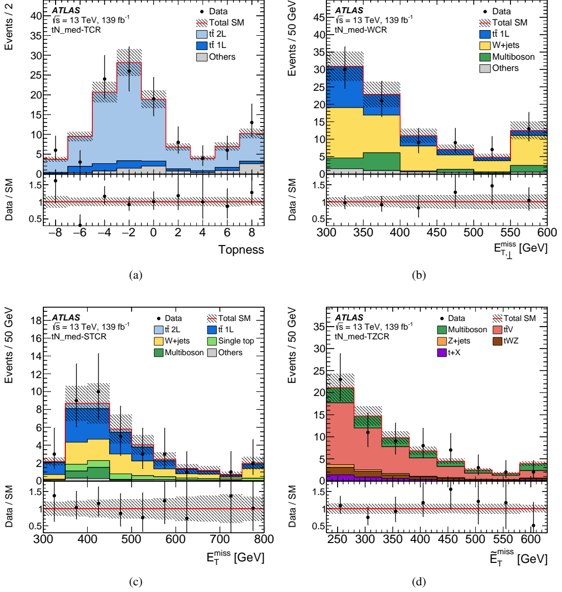
Figure 3: Selected kinematic distributions in t\bar{t}N_{\text{med}} CRs: (a) topness in the TCR, (b) E_{T,\perp}^{\text{miss}} in the WCR, (c) E_T^{\text{miss}} in the STCR, (d) \tilde{E}_T^{\text{miss}} in the TZCR. The distributions shown are post-fit, i.e. each background is scaled by a normalisation factor obtained from a background-only likelihood fit to the CRs (see Table 14). The hatched area around the total SM prediction and the hatched band in the Data/SM ratio include all statistical and systematic uncertainties. The last (first) bin contains overflows (underflows).
