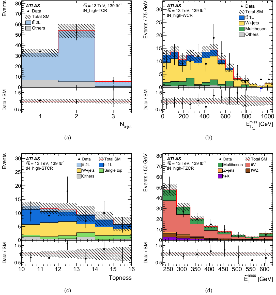
Figure 4: Selected kinematic distributions in tN_{\text{high}} CRs: (a) N_{b\text{-jet}} in the TCR, (b) E_{T,\perp}^{\text{miss}} in the WCR, (c) topness in the STCR, (d) \tilde{E}_T^{\text{miss}} in the TZCR. The distributions shown are post-fit, i.e. each background is scaled by a normalisation factor obtained from a background-only likelihood fit to the CRs (see Table 14). The hatched area around the total SM prediction and the hatched band in the Data/SM ratio include all statistical and systematic uncertainties. The last (first) bin contains overflows (underflows).
