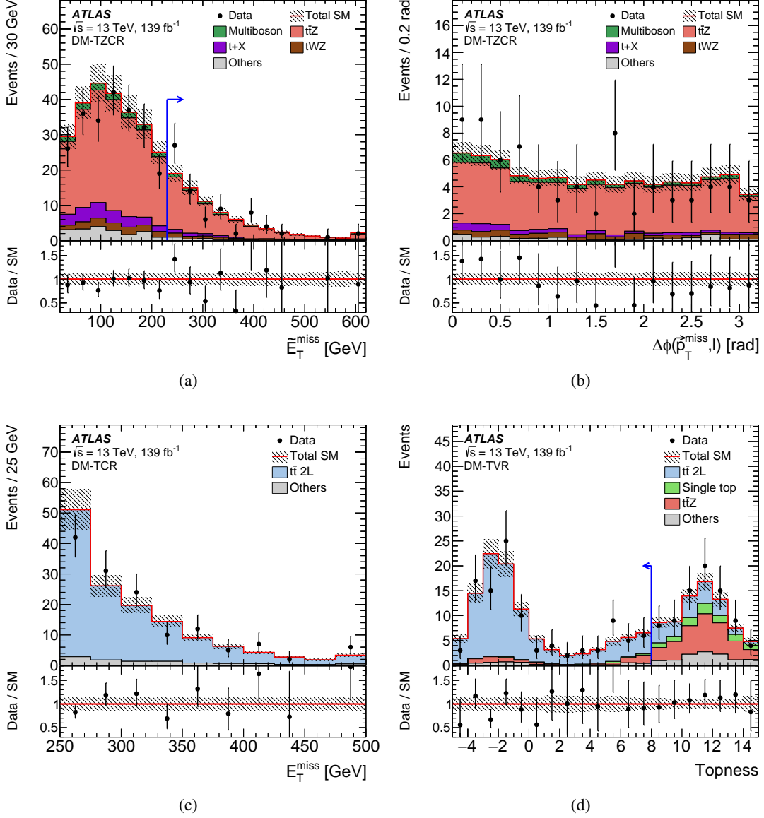
Figure 5: Selected kinematic distributions in DM CRs and VRs: (a) \tilde{E}_T^{\text{miss}} in the TZCR before applying the \tilde{E}_T^{\text{miss}} selection, (b) \Delta\phi(\vec{p}_T^{\text{miss}}, \ell) in the TZCR, (c) E_T^{\text{miss}} in the TCR, (d) topness in the TVR before applying the topness selection. For distributions where the requirement on the displayed variable is removed an arrow indicates the final selection on that variable. The distributions shown are post-fit, i.e. each background is scaled by a normalisation factor obtained from a background-only likelihood fit to the CRs (see Table 14). The hatched area around the total SM prediction and the hatched band in the Data/SM ratio include all statistical and systematic uncertainties. The last (first) bin contains overflows (underflows).
