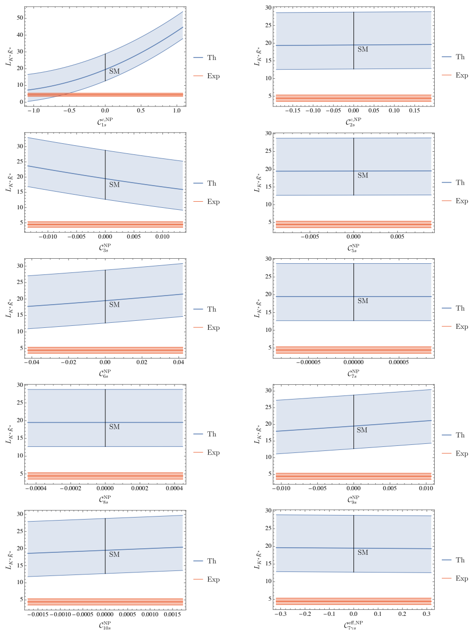
Figure 5. Sensitivity of L_{K^*\bar{K}^*} to individual contributions of NP in all different C_{is}^{NP} . For each coefficient, the range of variation considered for the NP contribution corresponds to 100% of its SM value.
