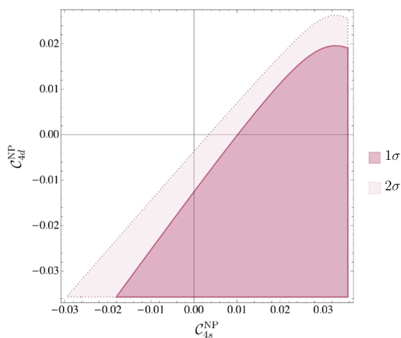
Figure 2. 1\sigma and 2\sigma CL regions from L_{K^* \bar{K}^*} allowing NP contributions to both C_{4s} and C_{4d} .
