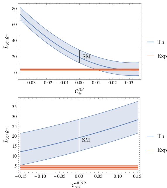
Figure 1. The tension between the theoretical prediction (blue) and the experimental value (orange) is reduced below 1\sigma for C_{4s}^{NP} \simeq 0.25C_{4s}^{SM} (upper plot) or C_{8gs}^{eff,NP} \simeq -C_{8gs}^{eff,SM} (lower plot). The predictions are given for C_{4s}^{NP} and C_{8gs}^{eff,NP} for a range corresponding to 100% of their respective SM values. The plots for the remaining Wilson coefficients can be found in appendix C.
