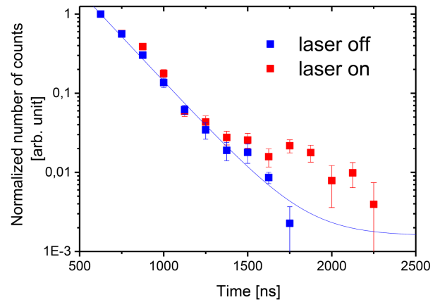
Fig. 3. Normalized number of gamma rays counted by the LaBr 3 (Ce) scintillator in the stopper region (30 cm far from the converter) with and without the laser pulse. The continuous line is a guide for the eyes.
