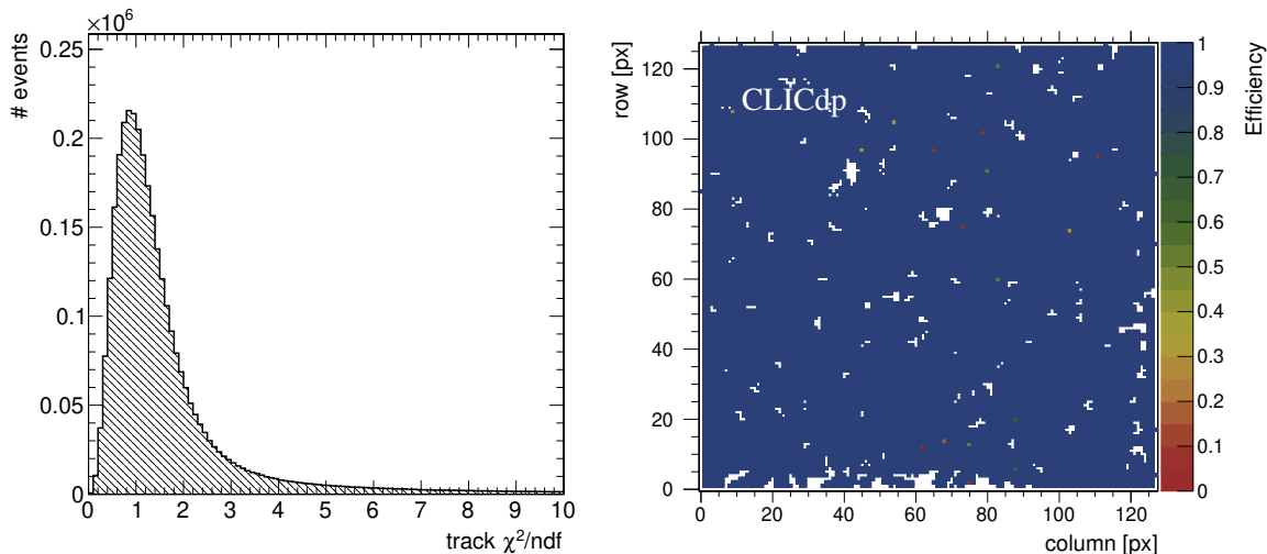
(a) Track \chi^2 divided by the number of degrees of freedom, provided by the Tracking4D module. (b) Efficiency as a function of the track position over the full chip area, masked areas appear white.
