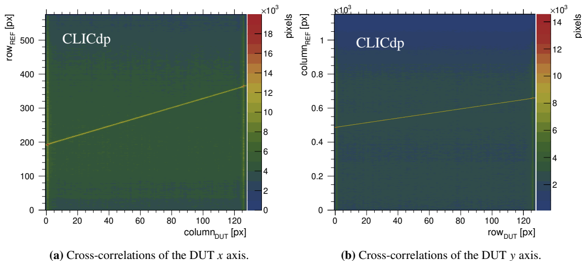
Figure 12. Cross-correlations between CLICpix2 (DUT) and the last upstream telescope plane (REF) in x (a) and y (b). The two detectors are rotated by 90^\circ with respect to each other, which makes it necessary to compare opposite coordinates (columns versus rows). These plots are provided by the Correlations module.
