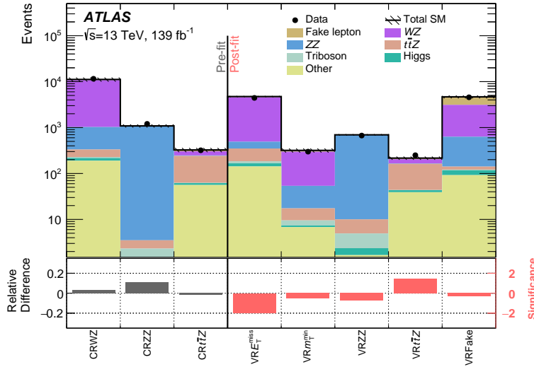
Figure 5: The observed data and the SM background expectation in the CRs (pre-fit) and VRs (post-fit). The “Other” category consists mostly of the tWZ , t\bar{t}W , and tZ processes. The hatched bands indicate the combined theoretical, experimental, and MC statistical uncertainties in the background prediction. The bottom panel shows the fractional difference between the observed data and expected yields for the CRs and the significance of the difference for the VRs, computed following the profile likelihood method described in Ref. [102].
