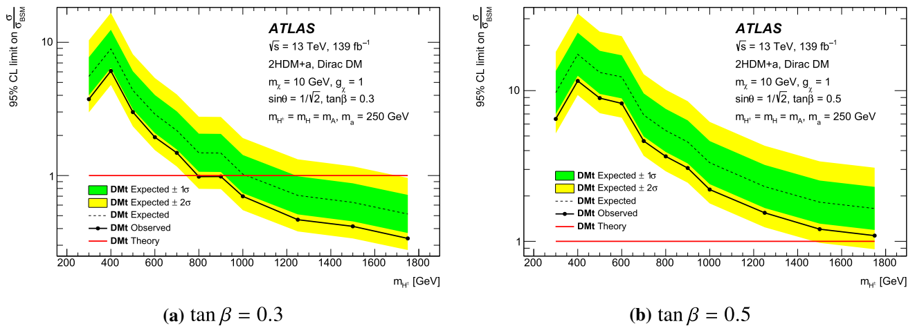
Fig. 15 The expected and observed cross-section exclusion limits as a function of m_{H^\pm} in the tj_{1L} analysis channel for signal models with m_a = 250 GeV, and a \tan\beta = 0.3 and b \tan\beta = 0.5 . The theoretical cross section of the t -channel DM production process is denoted by ‘Theory’
