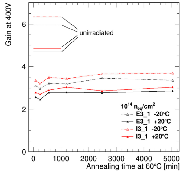
Fig. 2. Charge gain at 400 V as a function of annealing time at 60 °C. The gain is calculated using RF-TCT measurements, comparing the PIN diode and the LGADs in the same annealing state. Measurements before irradiation are shown as horizontal lines.
