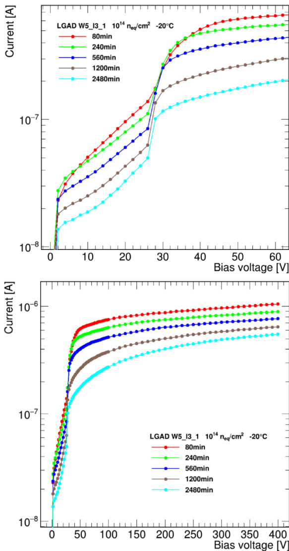
Fig. 3. Leakage current of LGAD W5_I3_1 as a function of bias voltage at -20\text{ }^{\circ}\text{C} for different annealing times. The data is shown in a limited voltage range (top) and in the full range (bottom).
