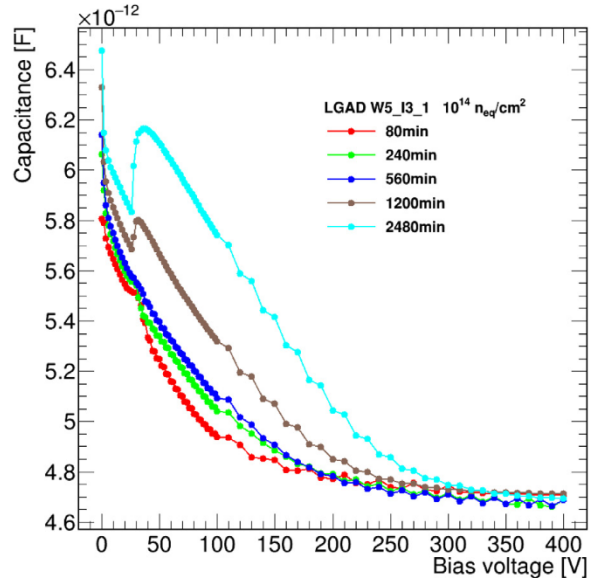
Fig. 9. Capacitance as a function of bias voltage for LGAD W5_I3_1 at different annealing states. CV measurements were carried out at 10 kHz with an alternating voltage amplitude of 0.5 V. The data is shown in a limited voltage range (top) and in the full range (bottom).
