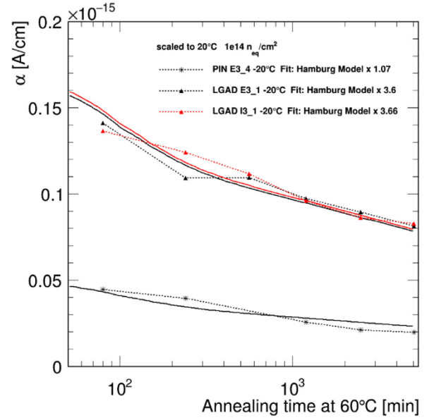
Fig. 11. Current related damage rate as a function of annealing time for both LGADs and the PIN diode. The respective fit by Eq. (5) is shown as a solid line. The measurements were performed at -20 \text{ }^\circ\text{C} and scaled to +20 \text{ }^\circ\text{C} .
