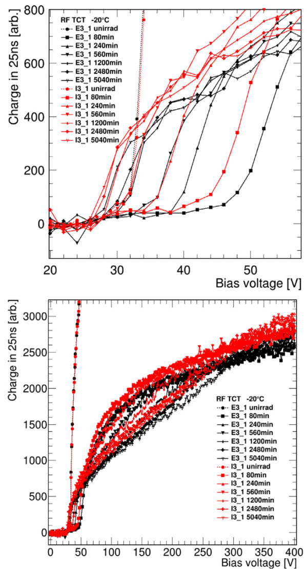
Fig. 4. Collected Charge in 25 ns with RF-TCT as a function of bias voltage for both LGADs, depicted in red and black, at different annealing times. The shown measurements were performed at -20\text{ }^{\circ}\text{C} . Measurements before irradiation are depicted as dashed lines. The data is shown in a limited voltage range (top) and in the full range (bottom).
