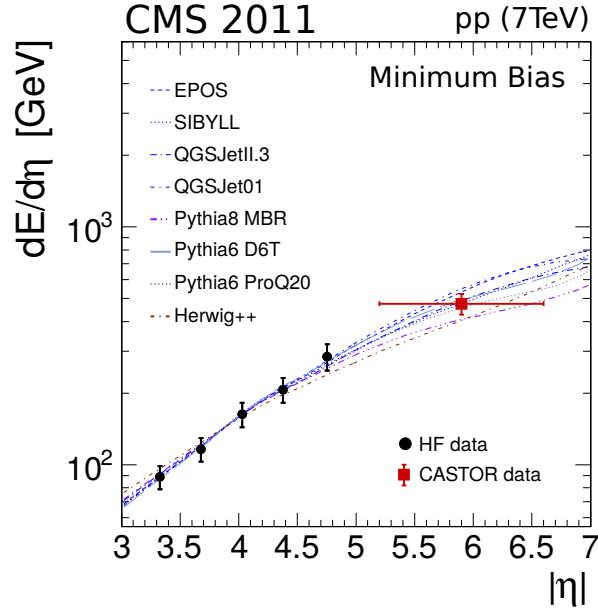
Figure 21: Pseudorapidity dependence of the forward energy flow in pp collisions at \sqrt{s} = 7 TeV measured in HF [15] and CASTOR, compared to MC simulations extrapolated to CASTOR. The uncertainties on the data are dominated by systematic effects. For the CASTOR datum the horizontal error bar indicates the \eta range of the calorimeter.
