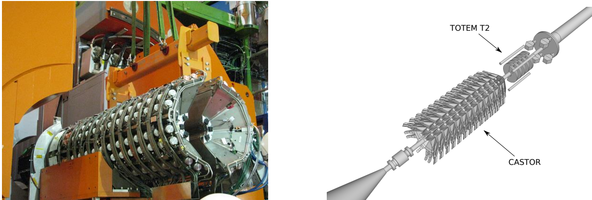
Figure 2: Left: Closeup image of the CASTOR calorimeter surrounded by the CMS collar shielding in the open position during an integration test, about 5 m below the beam pipe. Right: Visualization of the CASTOR detector integrated around the beam pipe. The CMS interaction point is at 14.4 m upstream (towards the upper right). The TOTEM T2 tracking station, and several pieces of LHC/CMS infrastructure, are visible along this direction.
