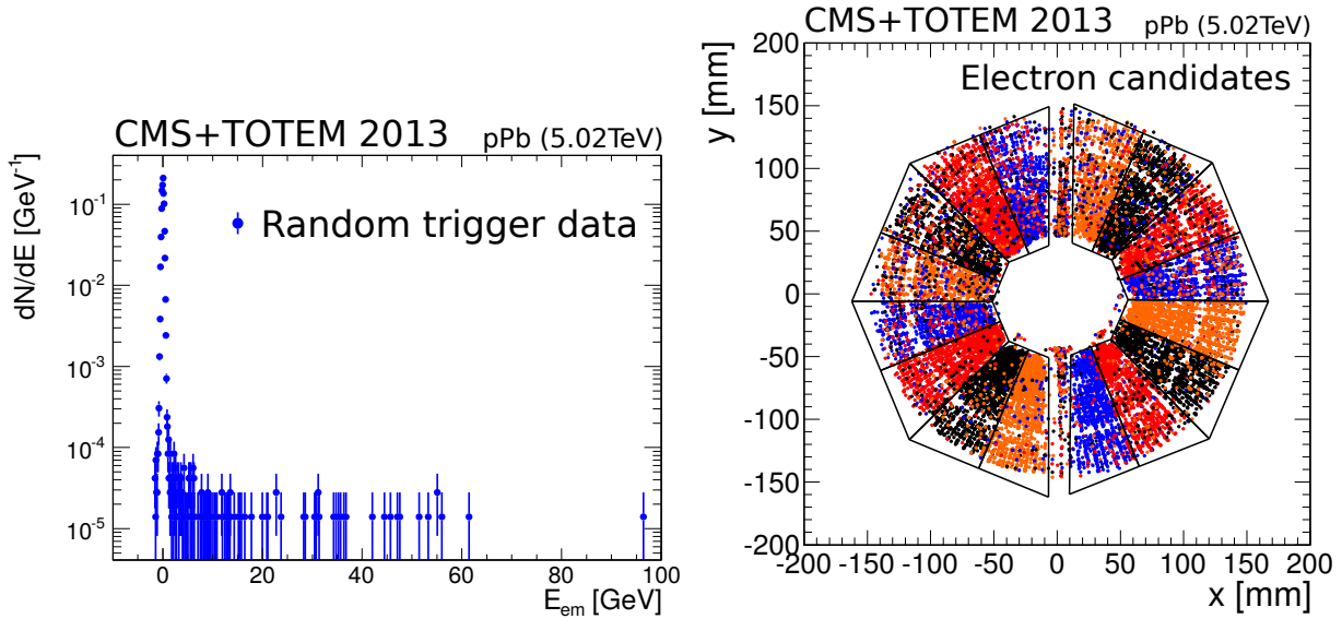
Figure 25: Left: Noise distribution of e.m. clusters in data used for the alignment of CASTOR with TOTEM T2 tracks, measured with a random trigger in pPb events with no collisions [66]. The RMS of the distribution is <1 GeV; the uncertainties are statistical only. Right: Projected (x,y) coordinates of single isolated T2 tracks onto the CASTOR front surface [66]. Only tracks (electron candidates) that coincide with a single isolated e.m. cluster in CASTOR are plotted. The points are colored alternatively depending on which calorimeter tower has registered the deposited energy. The black contours indicate the optimal positions of the two halves of CASTOR as derived from the analysis of these data. The empty ring at a radius of about 110 mm is caused by the shadow of a conical beam pipe section.
