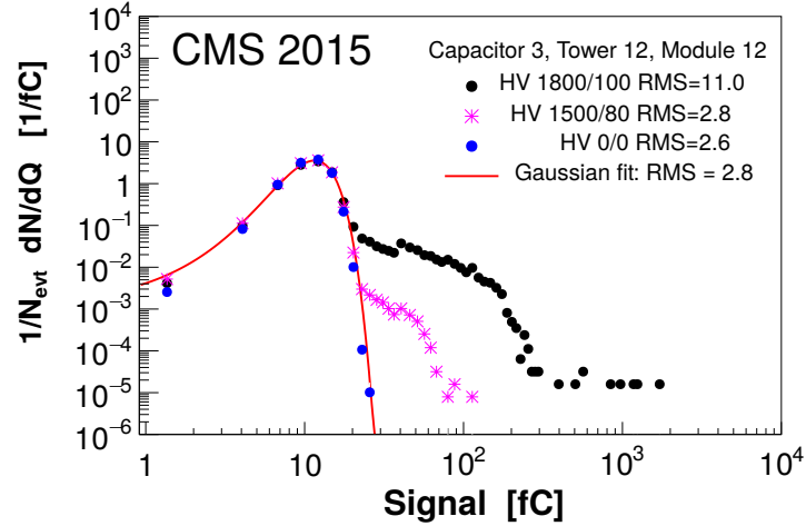
Figure 12: Charge spectrum for the noisiest capacitor of a typical CASTOR channel (tower 12, module 12) for various cathode/last dynode voltage settings (1800/100, 1500/80, and 0/0 V). A Gaussian fit to the data recorded with 0 V is also shown.
