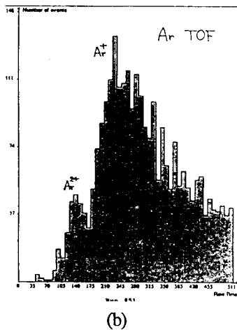
Fig. 5 Measured ion data in FFTB test[12]. (a) Azimuthal distribution of \text{He}^+ ions. (b) Time of flight spectrum obtained with Argon gas.
