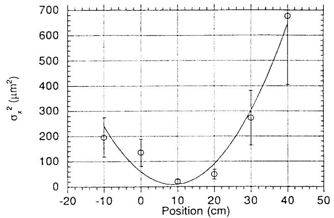
Fig. 6 Waist scan: Correlation between the distance to the waist and the measured dimension[12].
