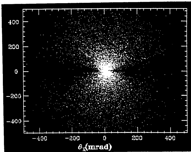
Fig. 10. Distribution of deflected electrons for JLC. Simulation by ABEL for the spot-size of \sigma_x = 260 nm, \sigma_y = 3.4 nm.
