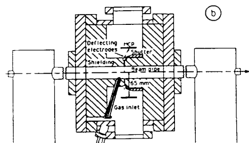
Fig. 4 Schematic view of gas-ionization beam-size monitor[11].
