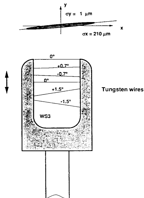
Fig.1. Specially arranged wire scanner for a very flat beam of intermediate focal point in FFTB[6].
