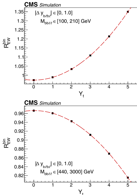
FIG. 6. The EW correction rate modifier R_{EW}^{\text{bin}} in two separate ( M_{bb\ell\ell}, \Delta y_{b\ell\ell} ) bins from simulated 2017 data, demonstrating the quadratic dependence on Y_t . All bins have an increasing or decreasing quadratic yield function, with the steepest dependence on Y_t found at lower values of M_{bb\ell\ell} .
