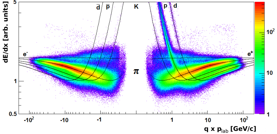
Figure 2: Example distribution of charged particles in the dE/dx – q \cdot p_{\text{lab}} plane in p+p interactions at 80 GeV/c. Expectations for the dependence of the mean dE/dx on p_{\text{lab}} for the considered particle types are shown by the curves calculated based on the Bethe-Bloch function.
