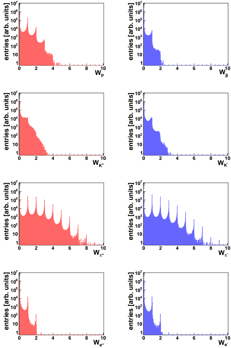
Figure 13: Smearing multiplicity distributions of positively ( left ) and negatively ( right ) charged particles (from top to bottom : p , K , \pi , e ) in p+p interactions at 158 GeV/c.
