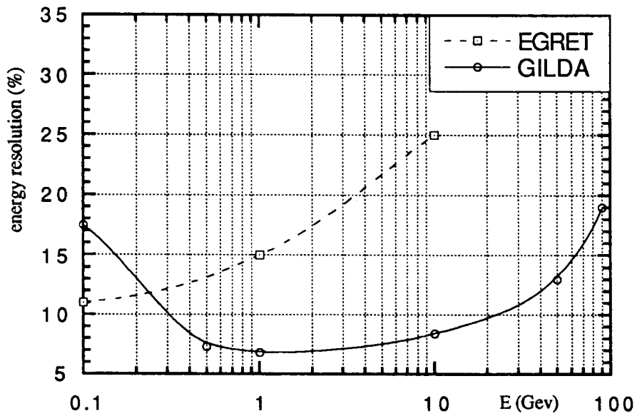
Figure 8: Simulated GILDA energy resolution, compared with EGRET.
