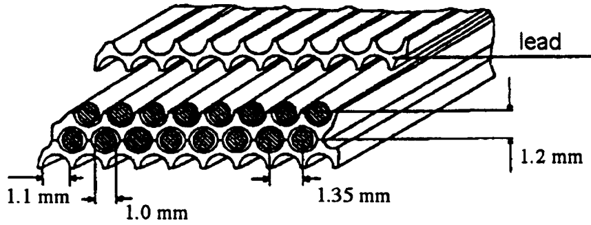
Figure 4: Structure of the lead scintillating fibers.
