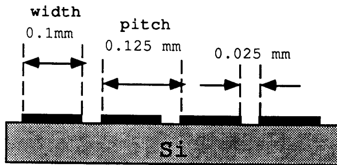
Figure 2: The 125 micron silicon strips.
