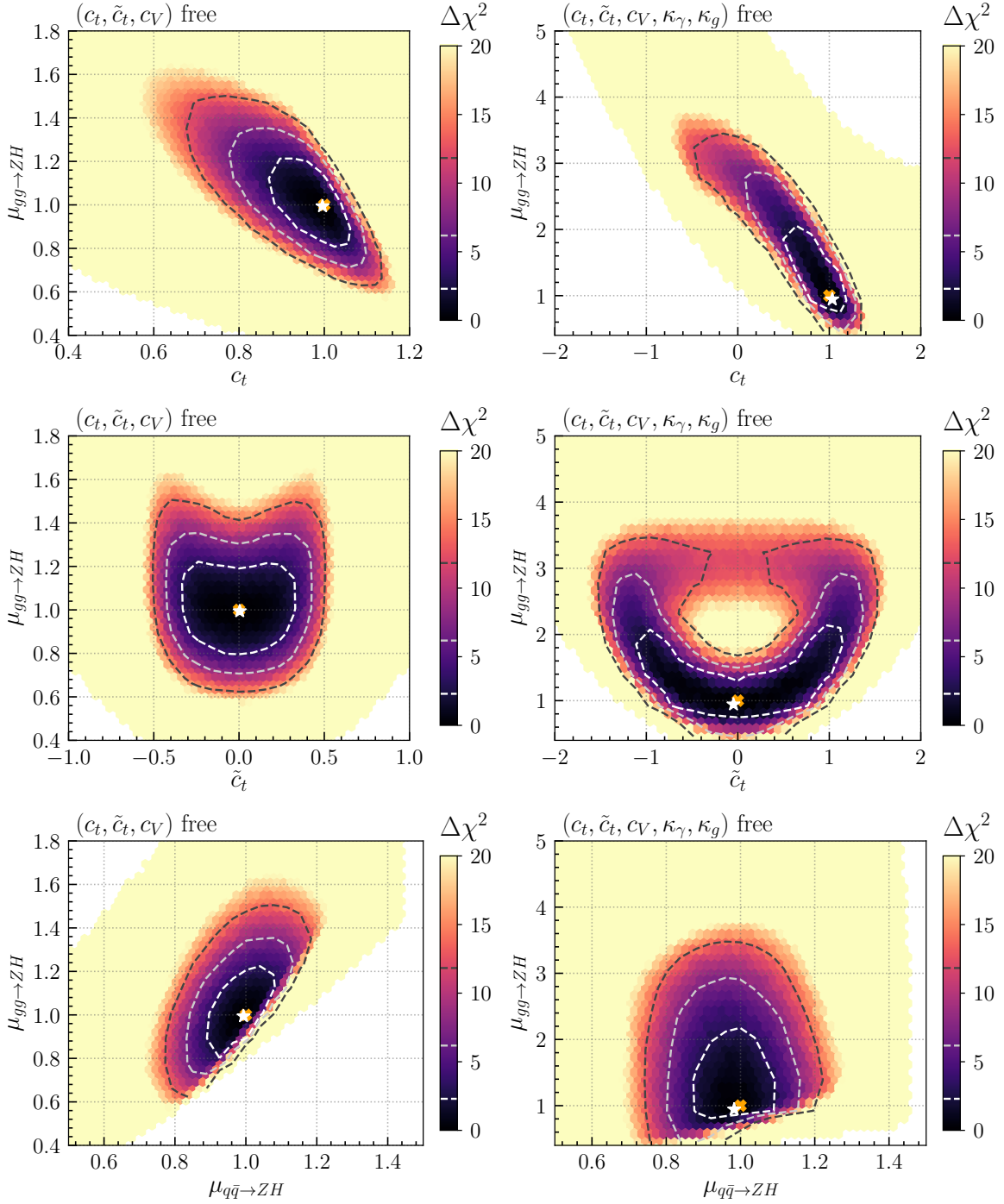
Figure 10. Predicted signal strength of gluon-initiated ZH production, \mu_{gg \rightarrow ZH} , in dependence of c_t ( top row ) and \tilde{c}_t ( middle row ) and its correlation with the q\bar{q} \rightarrow ZH signal strength, \mu_{q\bar{q} \rightarrow ZH} , ( bottom row ) for the 3D parametrization ( left panels ) and the 5D parametrization ( right panels ). The color corresponds to the profile \Delta\chi^2 of the global fit, and the 1\sigma , 2\sigma and 3\sigma confidence regions are shown as white, light-gray and dark-gray dashed contours, respectively. The best-fit point and the SM case are marked by a white star and an orange cross, respectively. Note the larger scale required to display the plots in the right panels.
