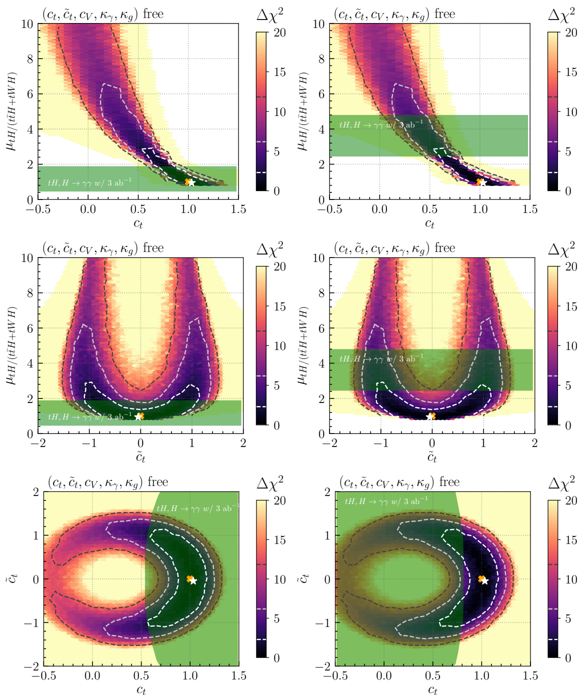
Figure 19. Impact of the prospective \mu_{tH}/(t\bar{t}H+tWH) determination of the proposed tH analysis with 3 \text{ ab}^{-1} of data [the green areas indicate the 1\sigma precision] on the currently allowed ranges of c_t (top panels), \tilde{c}_t (middle panels), as well as on the (c_t, \tilde{c}_t) parameter plane (bottom panels). The figures contain the fit results of the 5D parametrization shown in figure 13 (right panels) and figure 8 (bottom right panel), respectively. We assume the future \mu_{tH}/(t\bar{t}H+tWH) measurement to be consistent either with the SM (left panels) or the \mathcal{CP} -mixed 2 benchmark scenario (right panels).
