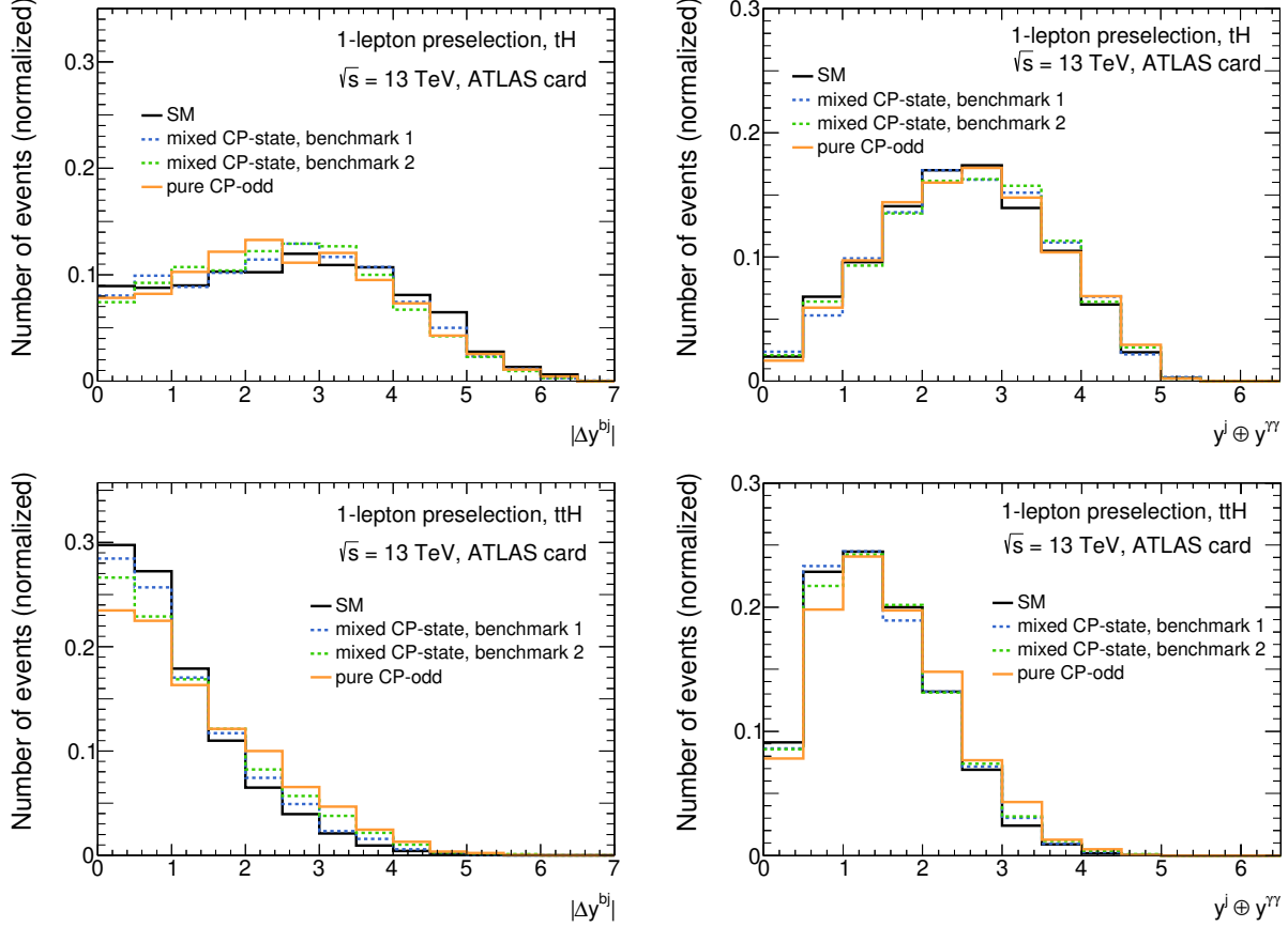
Figure 17: Comparison of the shape of (left) |\Delta y^{bj}| and (right) y^j \oplus y^{\gamma\gamma} in (top) tH and (bottom) t\bar{t}H production for the four \mathcal{CP} hypotheses considered in the study: SM, pure \mathcal{CP} -odd Higgs boson (solid lines), and two benchmarks of \mathcal{CP} -mixed states described in the text (dashed lines). Events are reconstructed with the Delphes software using the modified ATLAS card described in the text, similar results are obtained when using the HL-LHC card.
