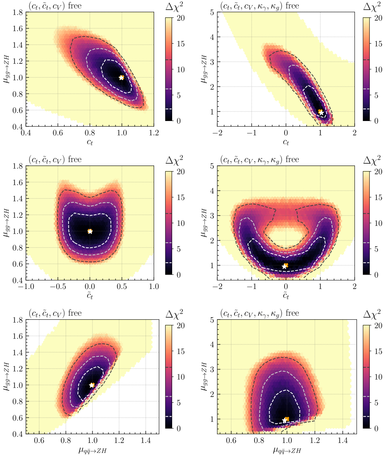
Figure 10: Predicted signal strength of gluon-initiated ZH production, \mu_{gg \rightarrow ZH} , in dependence of c_t (top row) and \tilde{c}_t (middle row) and its correlation with the q\bar{q} \rightarrow ZH signal strength, \mu_{q\bar{q} \rightarrow ZH} , (bottom row) for the 3D parametrization (left panels) and the 5D parametrization (right panels). The color corresponds to the profile \Delta\chi^2 of the global fit, and the 1\sigma , 2\sigma and 3\sigma confidence regions are shown as white, light-gray and dark-gray dashed contours, respectively. The best-fit point and the SM case are marked by a white star and an orange cross, respectively. Note the larger scale required to display the plots in the right panels.
