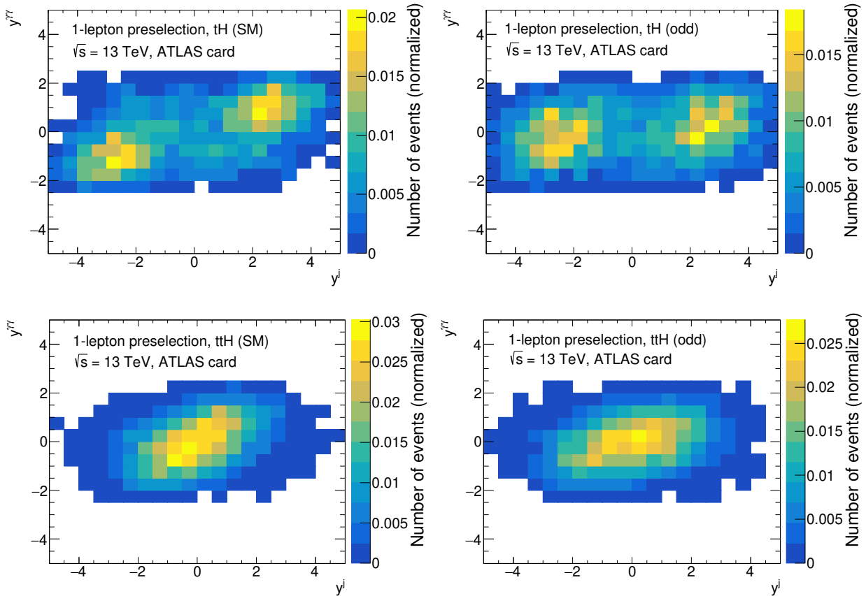
Figure 18: Comparison of the correlations between y^j and y^{\gamma\gamma} in (top) tH and (bottom) t\bar{t}H production in (left) the SM and (right) for a pure \mathcal{CP} -odd Higgs boson. Events are reconstructed with the Delphes software using the modified ATLAS card described in the text, similar results are obtained when using the HL-LHC card.
