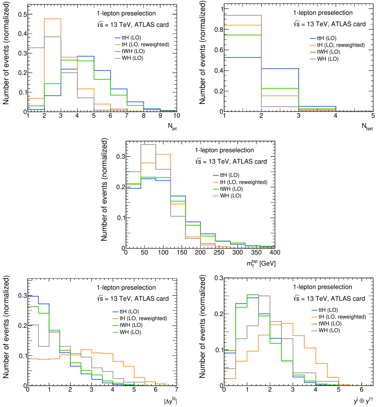
Figure 16: Comparison of the shape of (top, left) N_{jet} , (top, right) N_{bjet} , (middle) m_T^{top} , (bottom, left) |\Delta y^{bj}| and (bottom, right) y^j \oplus y^{\gamma\gamma} at LO+PS in SM tH , ttH , tWH and VH events passing the 1-lepton preselection. tH events are reweighted to match the NLO+PS N_{jet} shape. Events are reconstructed with the Delphes software using the ATLAS card described in the text, similar results are obtained when using the HL-LHC card.
