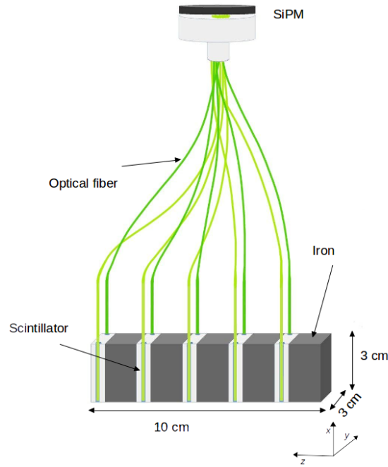
Figure 3: Layout of one LCM. The axis definition is the same as for Fig. 2
