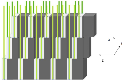
Figure 4: Layout of the fibers running toward the SiPMs through several LCMs by the iron grooves. The axis definition is the same as for Fig. 2
