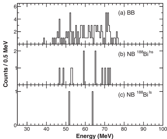
FIG. 3. Singles FF spectra from Si1 and Si2 for different RILIS modes: (a) BB mode; (b) NB( ^{188}\text{Bi}^{\text{hs}} ) mode; and (c) NB( ^{188}\text{Bi}^{\text{ls}} ) mode. Only calibration based on \alpha decays is used as a rough calibration, without any additional corrections; see text for details.
