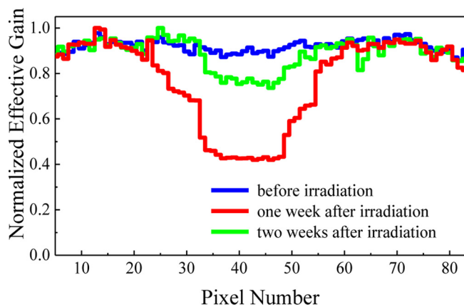
Fig. 3. Modification and evolution of the effective gain, gathered using low intensity ^{55}\text{Fe} source, of the moderately used detector under high intensity SXR radiation.
