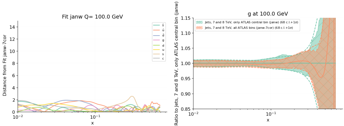
Figure 4.6. Same as Fig. 4.2, but now comparing the default most accurate fit to single-inclusive jet data (all datasets, NNLO QCD+EW, fit #janw), in which only the central rapidity bin of the ATLAS 7 TeV data is included, to a fit in which all rapidity bins are included (#janw-7cor). The gluon is shown as ratio to the former fit.
