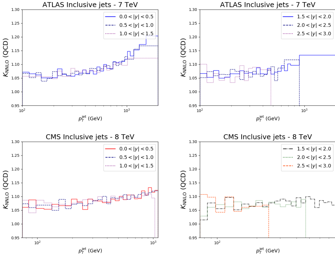
Figure 3.1. The NNLO QCD K -factors, Eq. (3.2), for the ATLAS 7 TeV (top) and CMS 8 TeV (bottom) single-inclusive jet cross-sections evaluated using NNPDF3.1 PDFs and scale \mu = \hat{H}_T . Results are shown as a function of the jet p_T in different jet rapidity bins, with the central (forward) bins shown in the left (right) plot.
