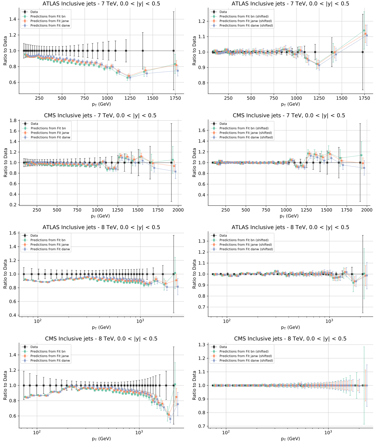
Figure 4.14. The theory to data ratio for a representative set of points from each single-inclusive jet dataset introduced in Sect. 2. Specifically, we show the central rapidity bins for all the ATLAS and CMS jet datasets at 7 and 8 TeV. Theoretical predictions are computed from fits #bn, #janw and #danw with corresponding theoretical accuracy, and shown as a ratio to the experimental data. For the data, either the full uncertainty is shown (left) or only the uncorrelated uncertainty, with the correlated uncertainty kept into account as a shift of the datapoint (right).
