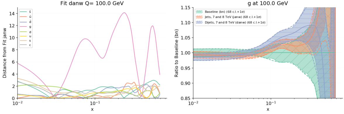
Figure 4.12. Same as Fig. 4.2, but now comparing the fits with all single-inclusive jet data ( \#janw ), and that with all dijet data ( \#danw ) and highest theory accuracy (NNLO QCD+ EW) and default settings. In the gluon comparison (right) results are displayed as a ratio to the baseline with no jet data included (also shown for reference).
