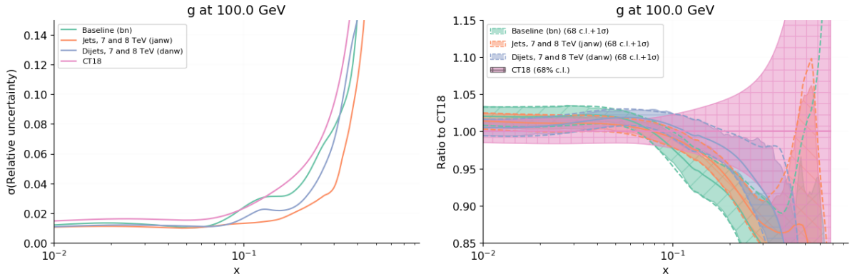
Figure 4.13. Same as Fig. 4.3, but now comparing the baseline ( \#bn ) to the fits with all single-inclusive jet ( \#janw ) and dijet data ( \#danw ) of Fig. 4.12. All results are shown as a ratio to the CT18 fit (also shown for reference).
