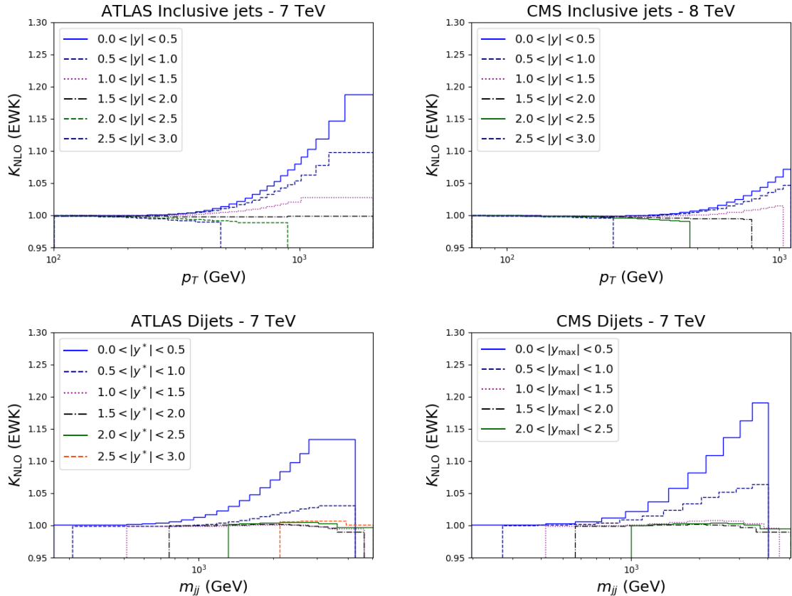
Figure 3.3. The EW K -factors, Eq. (3.3), for the ATLAS and CMS single-inclusive (top) and dijet (bottom) measurements. For single-inclusive jets the K -factors are shown as a function of jet p_T in six different rapidity bins. For dijets they are shown as a function of the dijet invariant mass m_{jj} for different y^* bins for ATLAS (left) or y_{\max} bins for CMS (right).
