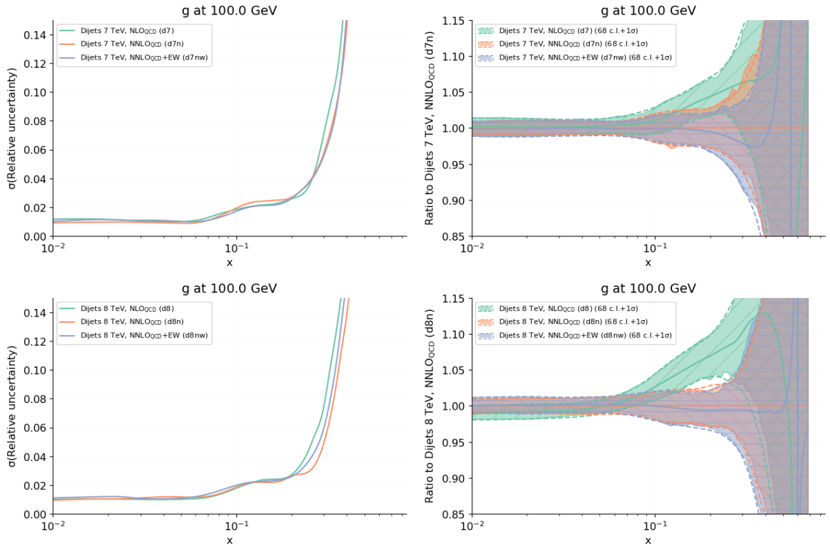
Figure 4.11. Same as Fig. 4.4, but now for dijets.
