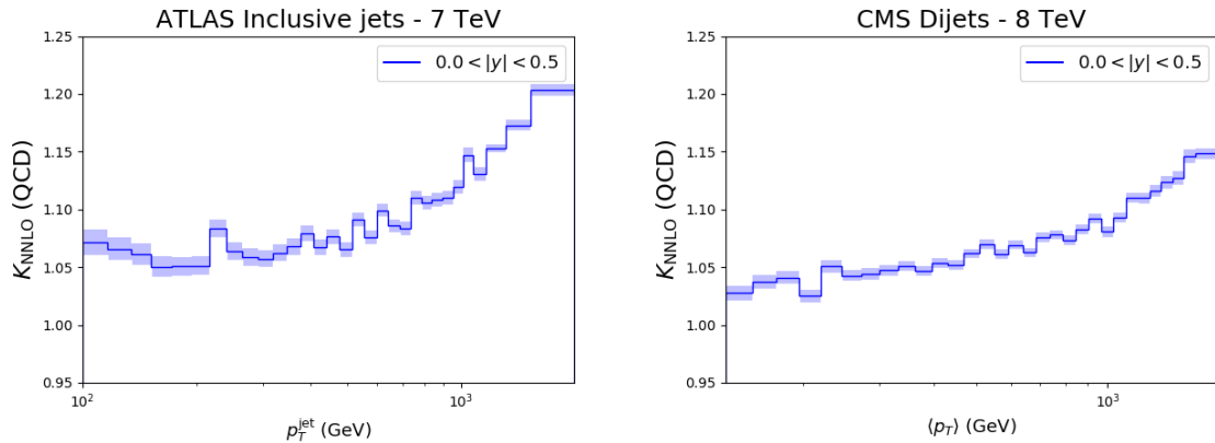
Figure 3.4. The NNLO QCD K -factors for the central rapidity bins of the ATLAS 7 TeV single-inclusive jets (left) and CMS 8 TeV dijets (right), with the Monte Carlo numerical uncertainties shown as filled bands around the central result.
