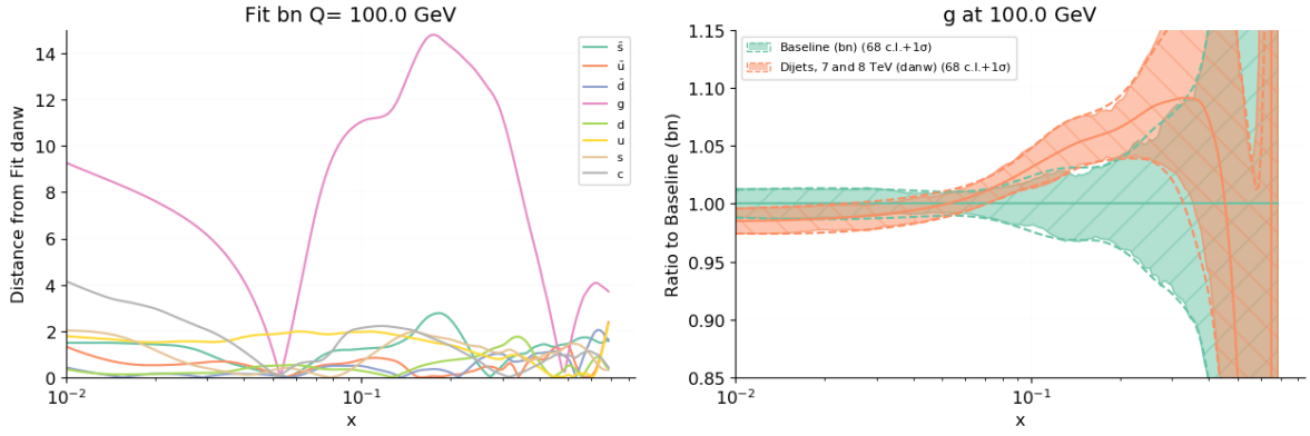
Figure 4.9. Same as Fig. 4.2, but now for dijets.
