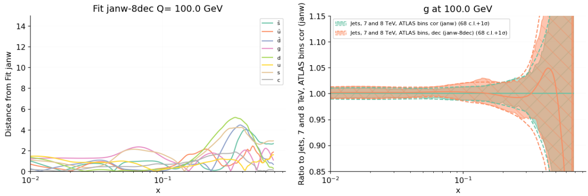
Figure 4.8. Same as Fig. 4.2, but now comparing the default most accurate fit to single-inclusive jet data (all datasets, NNLO QCD+EW, fit #janw), to a fit in which selected systematic uncertainties are decorrelated in the ATLAS 8 TeV data (fit #janw-8dec). The gluon is shown as ratio to the former fit.
