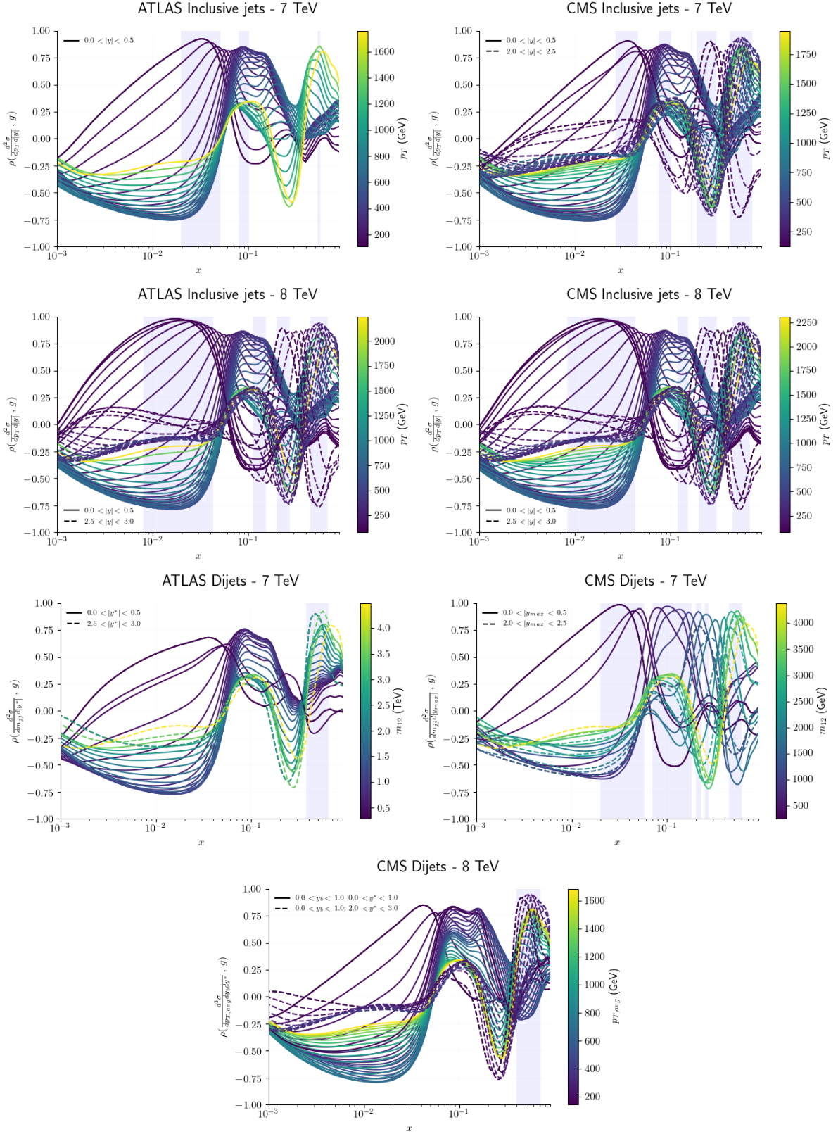
Figure 4.1. Correlation coefficients between the data of Table 2.1 and the gluon PDF g(x) . Each curve corresponds to a different datapoint, with the value of p_T corresponding to the color code on the right of the plot, and only curves for the points in the largest and smallest rapidity bins are shown. The shaded bands denote regions in which the maximum correlation is greater than 90% of the maximum correlation in the whole plot.
