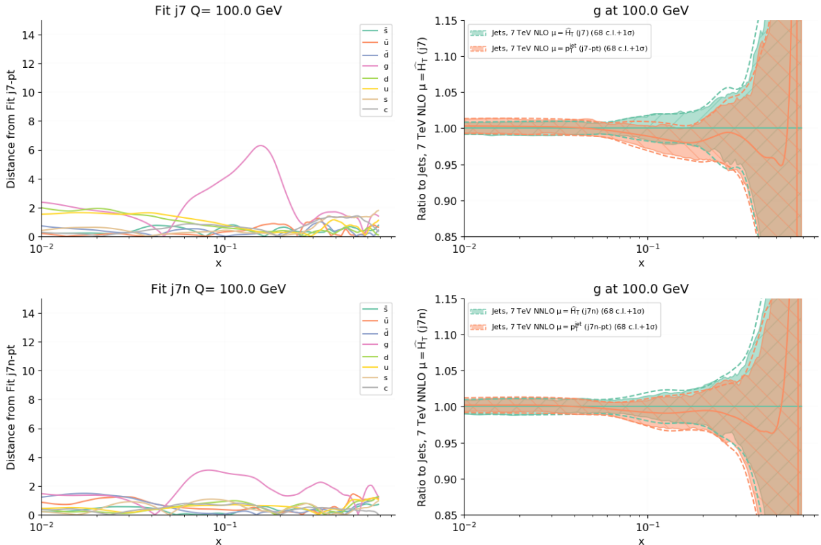
Figure 4.5. Same as Fig. 4.2, but now comparing fits to the 7 TeV data with the choices of central renormalization and factorization scale \mu = \hat{H}_T (as shown in Fig. 4.4, top) and \mu = p_T^{\text{jet}} at NLO (fits #j7 and #j7-pt) and NNLO (fits #j7n and #j7n-pt). The gluon is shown as ratio to the fits with \mu = \hat{H}_T .
