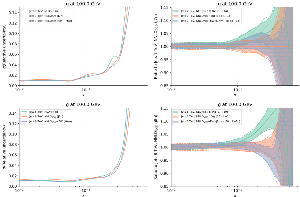
Figure 4.4. Same as Fig. 4.3, but now comparing fits with NLO, NNLO and NNLO+EW theory for 7 TeV (top: fits #j7, #j7n, #j7nw respectively) and 8 TeV (bottom: fits #j8, #j8n, #j8nw). All results are now shown as ratios to the NNLO fit.
