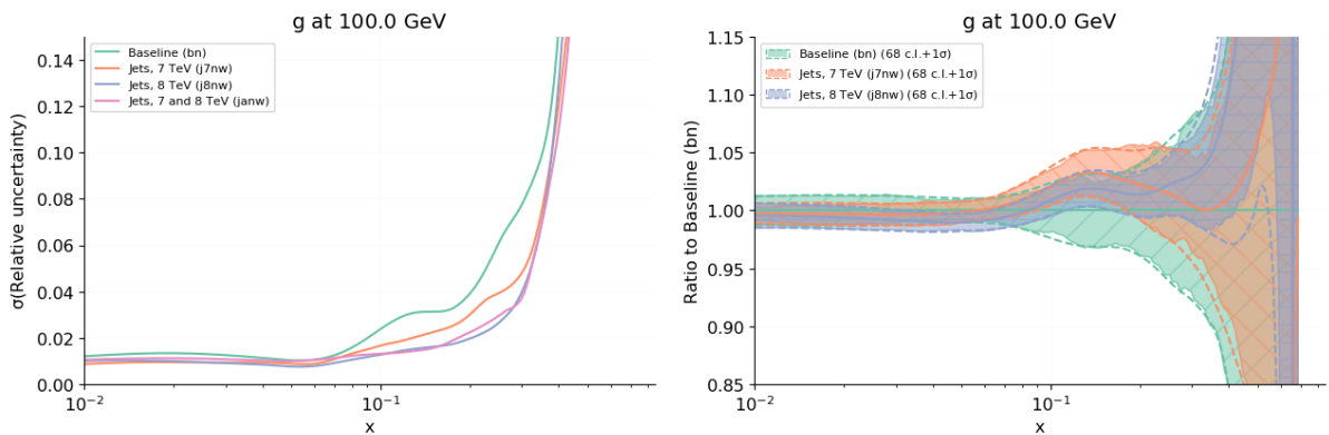
Figure 4.3. Comparison between the baseline fit with no jet data ( \#bn ), and the fits with only 7 TeV ( \#j7nw ) or only 8 TeV ( \#j8nw ) jet data included. The relative uncertainty on the gluon PDF (left) and the ratio of the gluon PDF to the baseline (right) are shown at Q = 100 GeV. All results are shown as ratios to the baseline.
