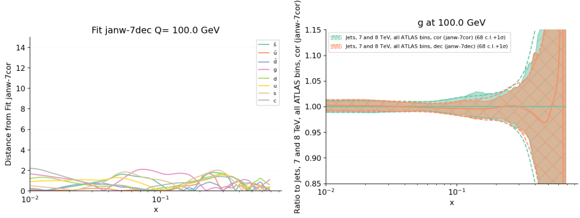
Figure 4.7. Same as Fig. 4.2, but now comparing the fits to single-inclusive jet data (all datasets, NNLO QCD+EW), in which all rapidity bins of the ATLAS 7 TeV data are included, either with (fit #janw-7cor) or without (fit #janw-7dec) experimental correlations on selected systematic uncertainties. The gluon is shown as ratio to the former fit.
