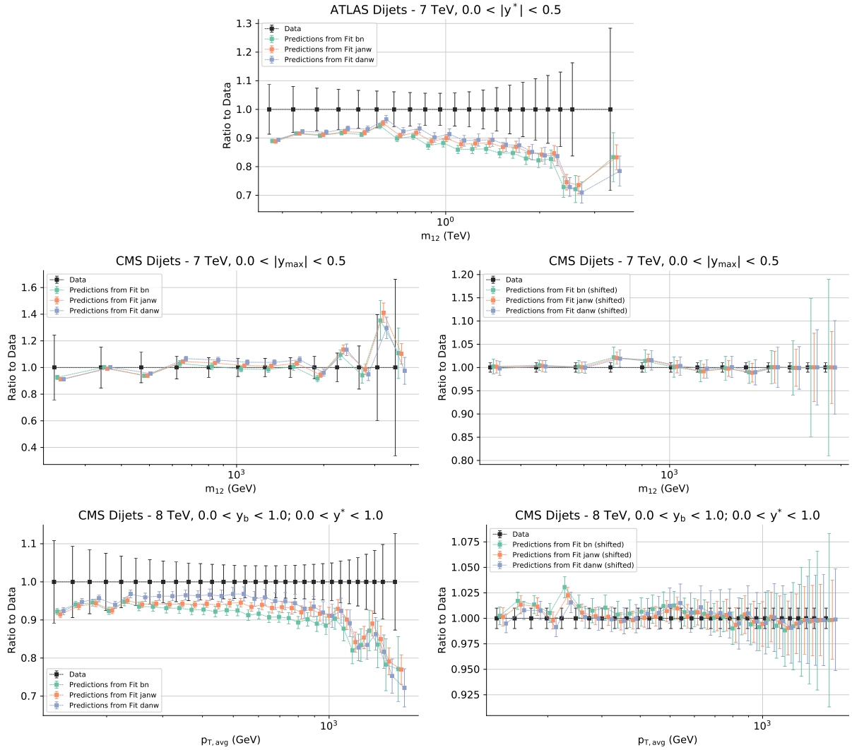
Figure 4.15. Same as Fig. 4.14, but for dijets. For the ATLAS data only the unshifted data are shown because the breakdown of the statistical covariance matrix into fully uncorrelated components is not available.
