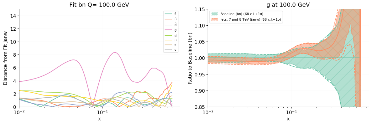
Figure 4.2. Comparison between the baseline fit with no jet data ( \#bn ) and the fit with all single-inclusive jet data included ( \#janw ), both with default settings and the most accurate theory (NNLO QCD, including EW corrections for jets). The distance (see text) between all PDFs (left) and the ratio of the gluon PDF to the baseline (right) are shown at the scale Q = 100 GeV. The shaded band is the 68% confidence interval, while the dashed lines are the edge of one sigma interval.
