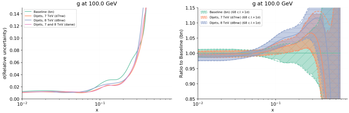
Figure 4.10. Same as Fig. 4.3, but now for dijets.
