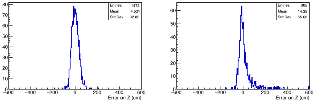
Figure 2. LArsoft evaluation of the precision on the localization of the actual neutrino vertex position, along the beam direction z , for \nu_e ( left ) and \nu_\mu ( right ) for the layout with 90 (8'') PMTs: a precision of about 30 cm (70 cm) for \nu_e CC ( \nu_\mu CC) is obtained.
