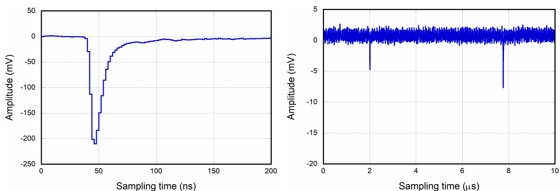
Figure 19. Left: example of actual PMT signal shape recorded in combination with a laser pulse. Right: a 10 μs off-light recording showing two random single photoelectron pulses.
