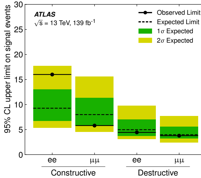
Figure 3: Model-independent upper limits at 95% CL on the number of signal events in the (constructive/destructive interference) SRs used in the analysis for dielectrons and dimuons.
