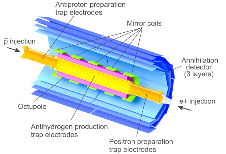
FIG. 1: Sketch of the ALPHA apparatus, showing the main components.
