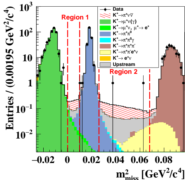
Figure 24: Reconstructed m_{\text{miss}}^2 distribution of data events with \pi^+ momentum between 15 and 35 GeV/c, passing the PNN selection (full symbols). The expected background and SM signal events contributions are superimposed as stacked histograms. The m_{\text{miss}}^2 distributions of the K^+ \rightarrow \pi^+\pi^0 , K^+ \rightarrow \mu^+\nu and K^+ \rightarrow \pi^+\pi^+\pi^- decays and of the upstream events are extracted from data. The other contributions are obtained from simulations.
