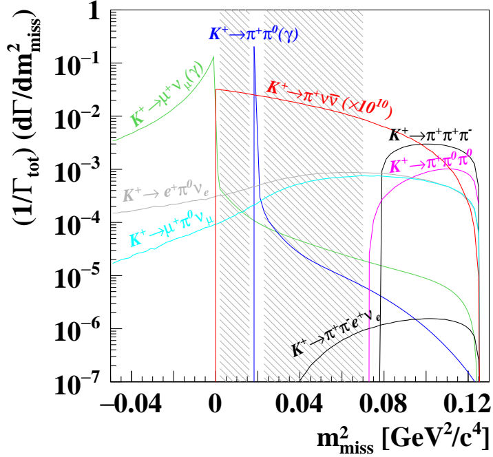
Figure 1: Expected theoretical distributions of the m_{\text{miss}}^2 variable relevant to the K^+ \rightarrow \pi^+ \nu \bar{\nu} measurement, before applying acceptance and resolution effects. The m_{\text{miss}}^2 is computed under the hypothesis that the charged particle in the final state is a \pi^+ . The K^+ \rightarrow \pi^+ \nu \bar{\nu} signal (red line) is multiplied by 10^{10} for visibility. The hatched areas include the signal regions.
