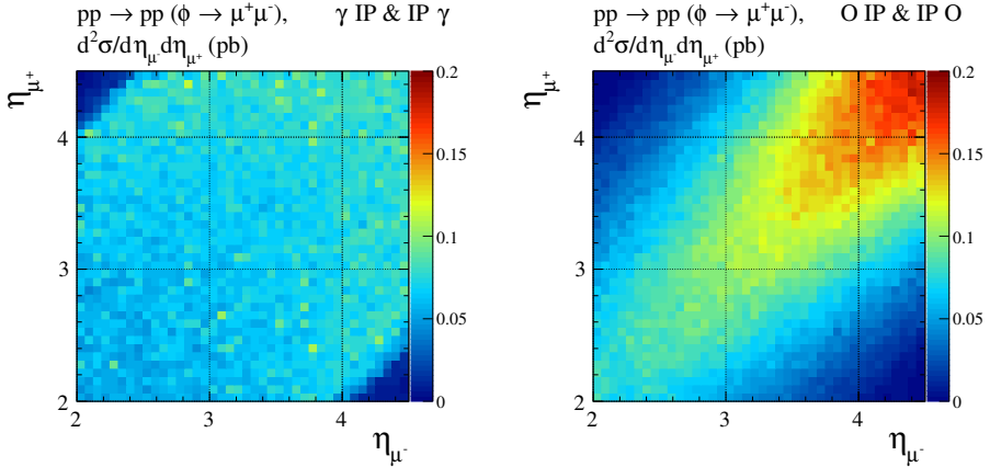
Fig. 7. The two-dimensional distributions in (\eta_{\mu^+}, \eta_{\mu^-}) for the pp \rightarrow pp\mu^+\mu^- reaction. Shown are the results for the \phi production via \gamma\text{-}\mathbb{P} fusion (left) and via \mathbb{O}\text{-}\mathbb{P} fusion (right). The calculations were done for \sqrt{s} = 13 TeV and with cuts on M_{\mu^+\mu^-} \in (1.01, 1.03) GeV, 2.0 < \eta_{\mu} < 4.5 , p_{t,\mu} > 0.1 GeV, and p_{t,\mu^+\mu^-} > 0.8 GeV.
