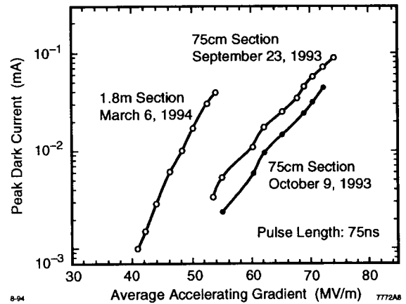
Fig. 10 Peak dark current measured by a downstream Faraday cup for the 75 cm constant-impedance and the 1.8 m detuned section as a function of average accelerating gradient.
