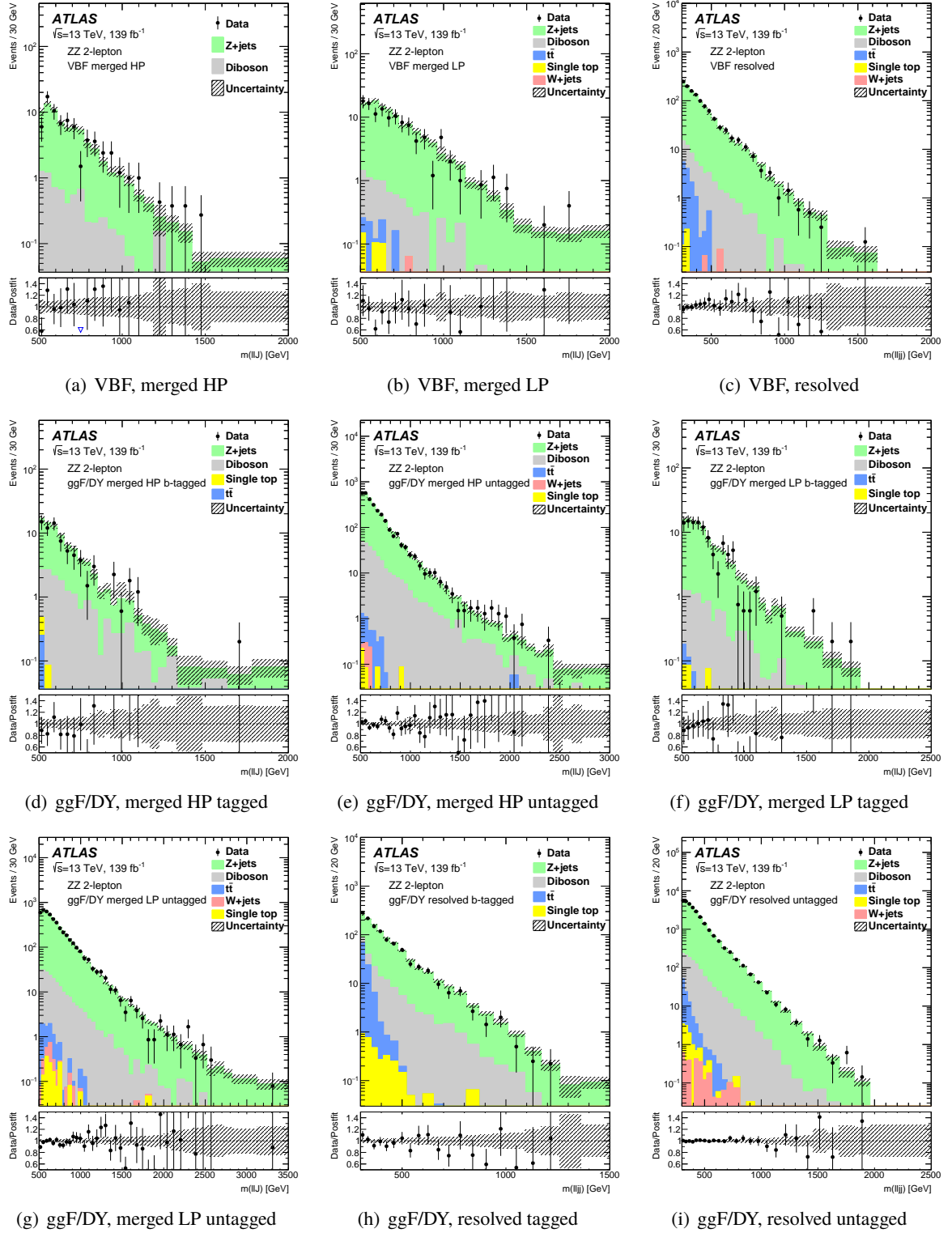
Figure 11: Comparisons of the observed data and the expected background distributions of m_{\ell\ell j} or m_{\ell\ell} in the 9 ZZ SRs of the 2-lepton channel. The background predictions are obtained through a background-only simultaneous fit to the 6 WW and 15 ZZ SRs and their respective V +jets and t\bar{t} CRs (see text). The bottom panes show the ratios of the observed data to the background predictions. The blue triangles indicate bins where the ratio is non-zero and outside the vertical range of the plot. The hatched bands represent the uncertainties in the total background predictions, combining statistical and systematic contributions.
