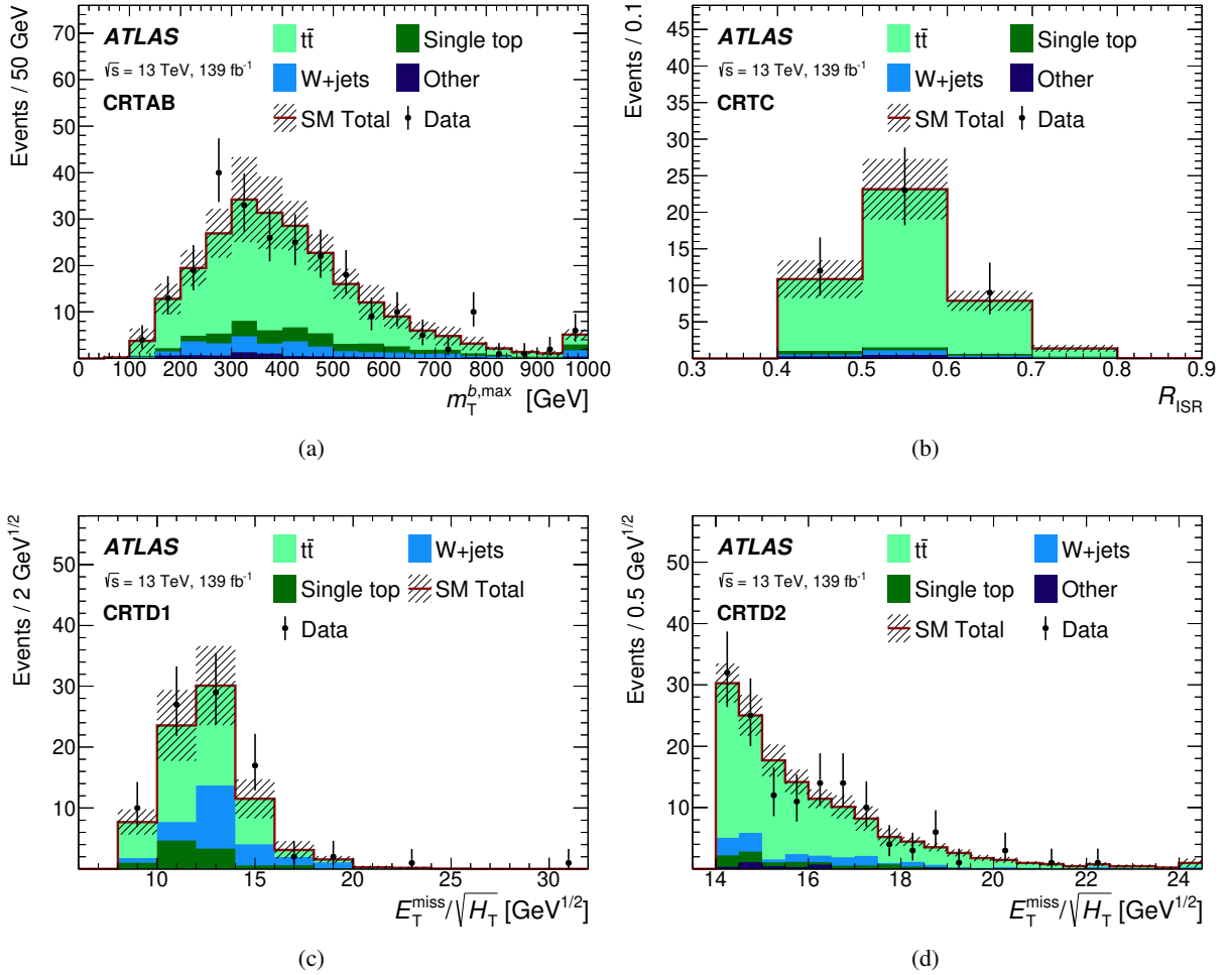
Figure 6: Distributions illustrating the level of agreement between data (points) and the SM expectation (stacked histogram, after simultaneously fitting to all backgrounds) in the t\bar{t} control regions: (a) m_T^{b,\text{max}} for CRTAB, (b) R_{\text{ISR}} for CRTC, and E_T^{\text{miss}}/\sqrt{H_T} for (c) CRTD1 and (d) CRTD2. The hatched uncertainty band around the SM expectation includes the combination of MC statistical, theory-related and detector-related systematic uncertainties. The rightmost bin in each plot includes all overflows.
