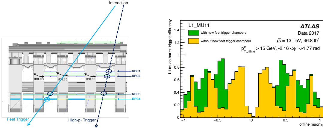
Figure 2: Left: Sketch showing the position of the new RPC chambers (RPC4) in the feet sectors. The muon trajectory on the left is accepted by a two-layer coincidence (RPC3-RPC4) using the new feet chambers. The trajectory on the right shows a muon accepted by the standard three-layer (RPC1-RPC2-RPC3) high- p_T trigger. Right: L1 trigger efficiency as a function of the pseudorapidity of offline reconstructed muon candidates in the barrel detector region for -2.16 < \phi < -1.77 evaluated for a trigger applying a 3-station coincidence requirement and a p_T threshold of 10 GeV (L1_MU11). The contribution of the newly installed RPC chambers is shown in green, while the remaining contribution is shown in yellow. Muons are required to pass Medium quality requirements [28] and have a transverse momentum of at least 15 GeV.
