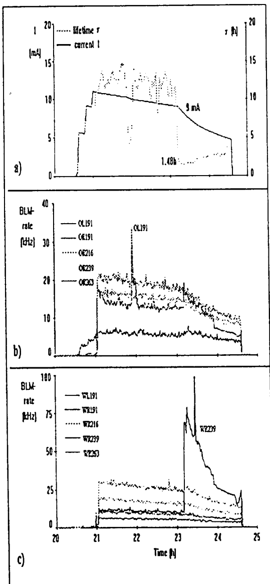
Figure 2: a) Electron beam current and lifetime versus time, b,c) response of selected BLMs in the east and in the west areas of HERA.
