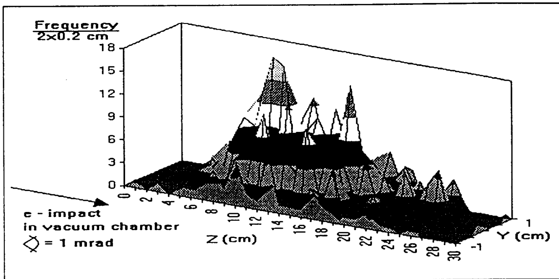
Figure 3: Shower leakage distribution (charged particles) on the side of the beam pipe surface. Z is the direction of the electron beam. The loss occurs at (z,y) = (0,0) . The wall thickness is 1 cm copper and 0.5 cm lead. The simulation is based on 202 primary electrons.
