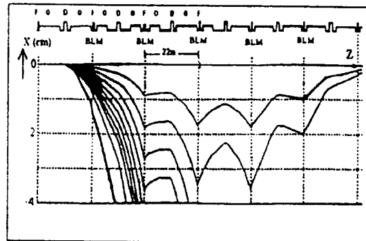
Figure 1: Path of electrons with an energy loss of \Delta E/E = -1\% to -10\% through a FODO structure. x is the horizontal displacement of the electrons. The pipe wall starts at x = \pm 4 \text{ cm} .
