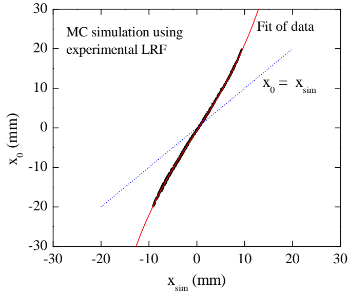
Figure 18: Direct SiPM-matrix readout: true coordinate of interaction point x_0 as a function of reconstructed coordinate x_{sim} (black dots), the latter obtained using MC simulation with the experimental LRF , and a fit of this dependence by polynomial function (red curve). For comparison, the dependence x_0 = x_{sim} is shown (blue dotted line)
