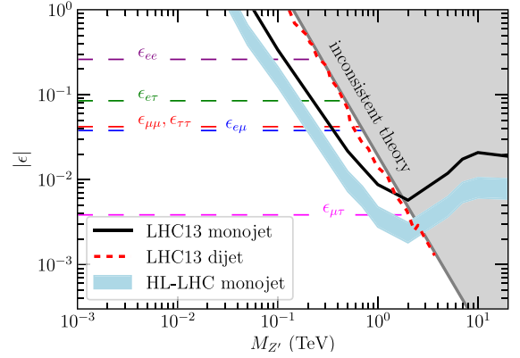
Fig. 1. Constraints on neutrino non-standard interactions from LHC data and neutrino experiments [27] as a function of the mediator mass M_{Z'} , assuming \epsilon_{\alpha\beta} \equiv \epsilon_{\alpha\beta}^u = \epsilon_{\alpha\beta}^d . Note that LHC constraints are independent of neutrino flavor. We assumed \Gamma_{Z'}/M_{Z'} = 0.1 here.
