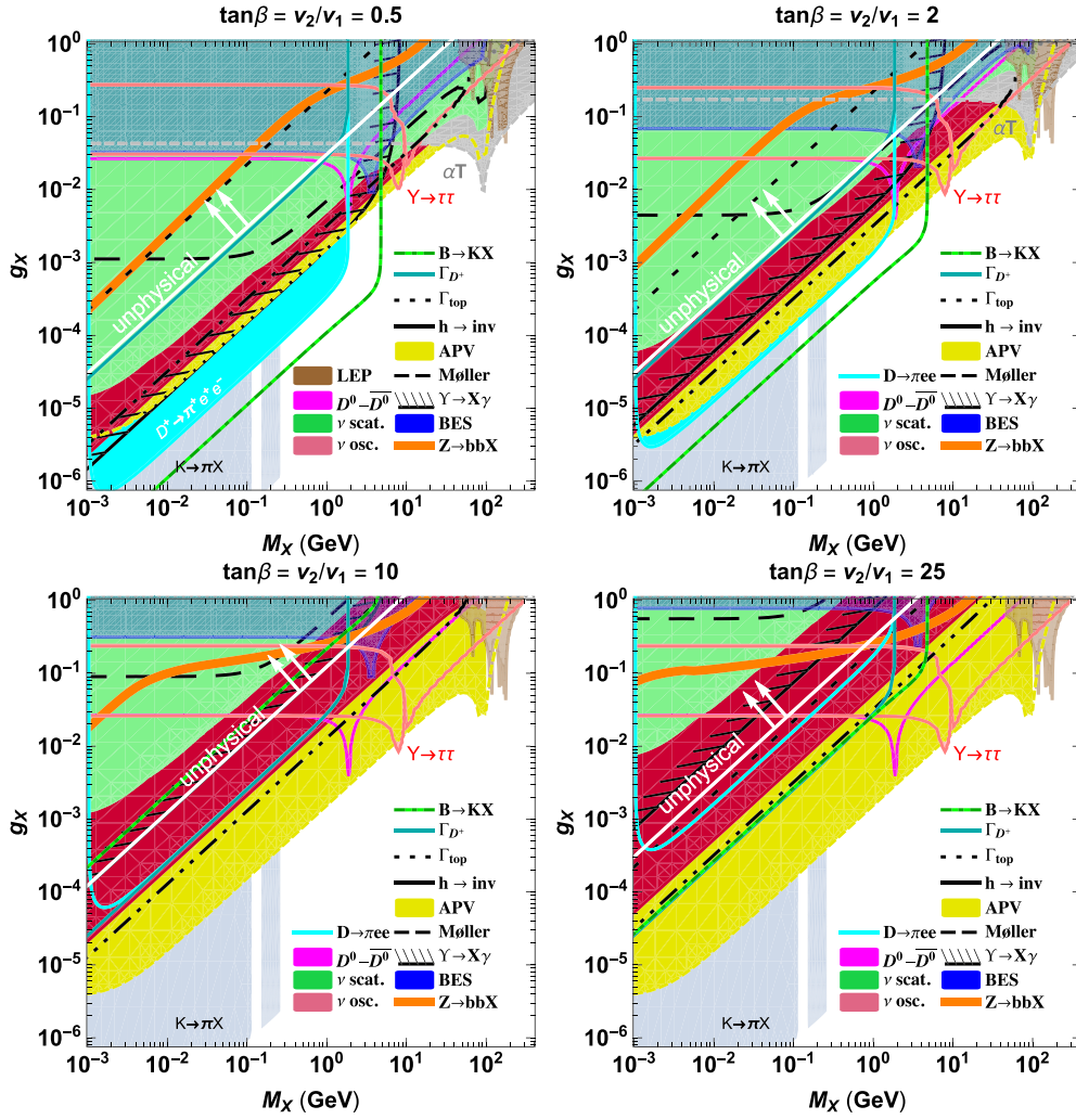
Fig. 5. Corrected constraints from Ref. [12] in the plane M_X versus g_X (gauge coupling) for various values of \tan\beta , as indicated. The constraints come from the following experiments or observations: B \rightarrow K +invisible (dark/light green); decay width of D^+ meson (dark cyan) and top quark (dotted line); Higgs invisible decays (dot-dashed line); atomic parity violation (APV, yellow); Möller scattering (dashed line); \Upsilon \rightarrow \gamma +invisible (hatched region); BES (blue region); Z \rightarrow bb +invisible (orange thick line); neutrino oscillations (red region) and scattering (green region); D^+ \rightarrow \pi^+ e^+ e^- (cyan); D - \bar{D} oscillation (magenta); electroweak T parameter (gray region); LEP data (brown region); K^+ \rightarrow \pi^+ +invisible (light blue region); and \Upsilon \rightarrow \tau^+ \tau^- decays (salmon line). The region above the white line labelled “unphysical” is forbidden for a given choice of \tan\beta . The differences with respect to Ref. [12] show up in the high M_X region.
