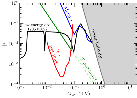
Fig. 4. Sensitivities to a specific UV complete model realization of non-standard interactions where the B - L number of the third family is gauged [12]. This includes current low energy observables (black), electroweak T parameter (green solid and dotted, see text), future high-luminosity LHC searches for bb\tau\tau final states (red, adapted from Ref. [40]), and LHC mono-jet searches (blue).
