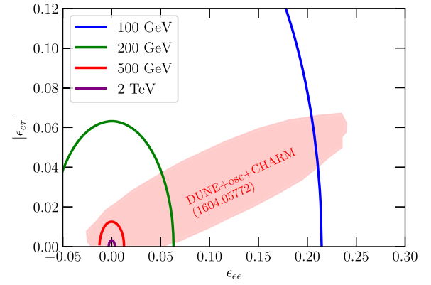
Fig. 2. Constraints on neutrino non-standard interactions from LHC data, for different mediator masses as labeled, with \Gamma_{Z'}/M_{Z'} = 0.1 , assuming \epsilon_{\alpha\beta} \equiv \epsilon_{\alpha\beta}^u = \epsilon_{\alpha\beta}^d . A fit to simulated data for DUNE from Ref. [37] is also included (pink shaded region).
