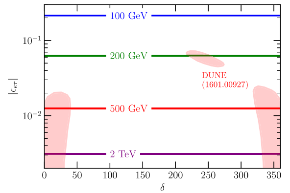
Fig. 3. An example of degeneracy in the (\epsilon_{e\tau}, \delta) plane, where \delta is the standard CP violating phase and \epsilon_{e\tau} \equiv \epsilon_{e\tau}^u = \epsilon_{e\tau}^d , from future DUNE data taken from Ref. [38] (pink shaded regions are allowed, assuming \epsilon_{e\tau} = \delta = 0 as null hypothesis). We overlay the LHC sensitivity to this NSI parameter for several mediator masses, as labeled, assuming \Gamma_{Z'}/M_{Z'} = 0.1 .
