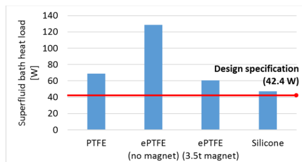
Figure 3. Heat load to Cluster D superfluid bath with different sealing configurations
