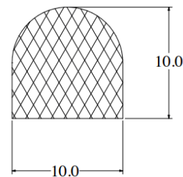
Figure 5. Silicone D-profile
