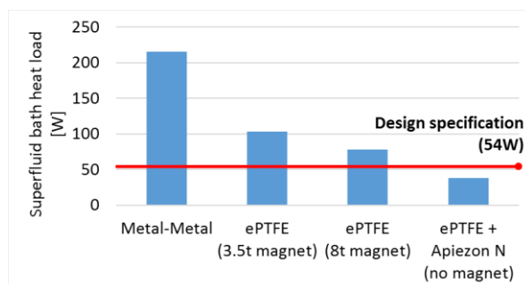
Figure 2. Heat load to HFM superfluid bath with different sealing configurations
