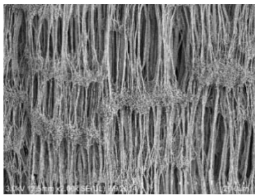
Figure 4. Microstructure of ePTFE (Gore®).
