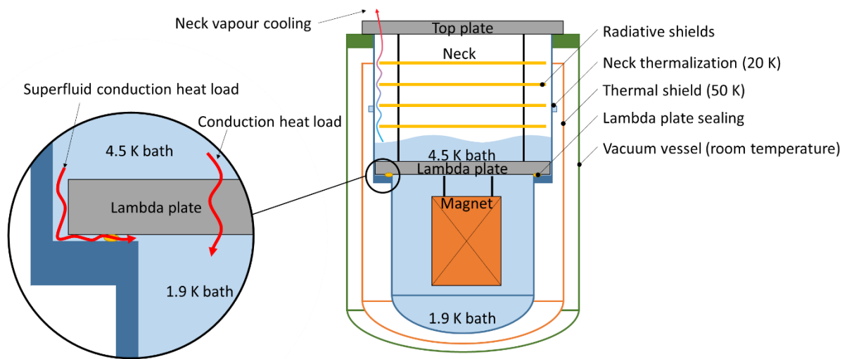
Figure 1. Schematic of a Vertical cryostat
