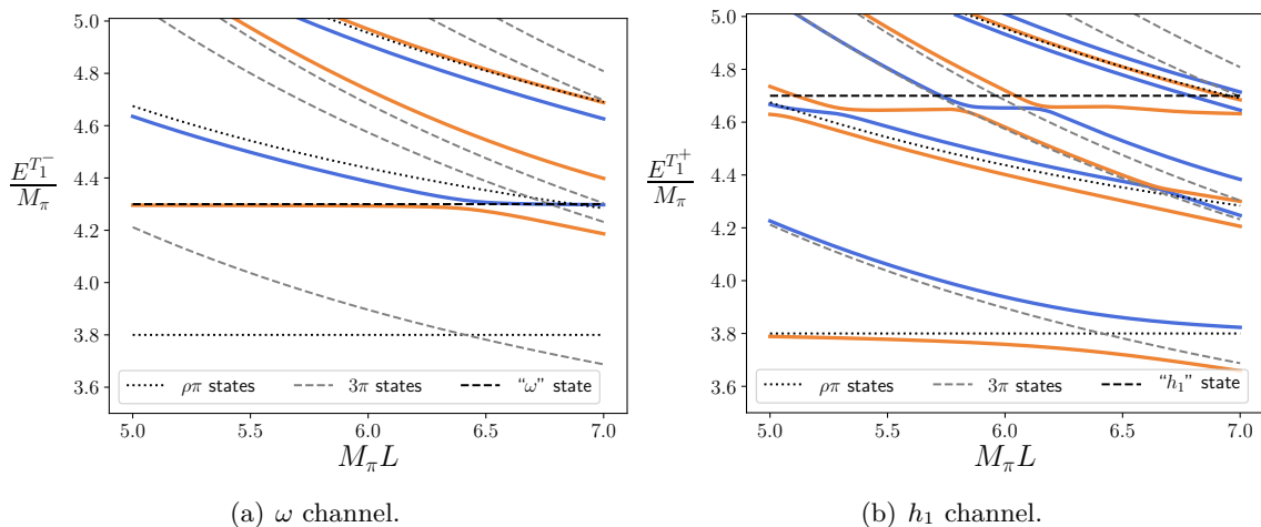
Figure 4: Illustrative finite-volume spectra for three pions with I_{\pi\pi\pi} = 0 and irreps (a) T_1^- and (b) T_1^+ , plotted versus M_\pi L . The interacting spectrum is shown by solid lines, with the alternating orange and blue colors only used to distinguish adjacent levels. Dashed and dotted grey lines show the comparison with different noninteracting levels. The parameters used for \mathcal{K}_2 and \mathcal{K}_{\text{df},3} are described in the text.
