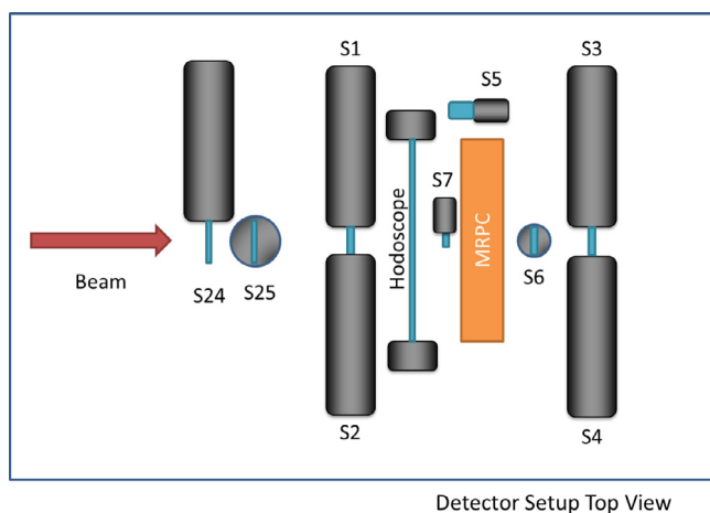
Fig. 2. The experimental setup for MRPC test in the ELBE test beam facility.
