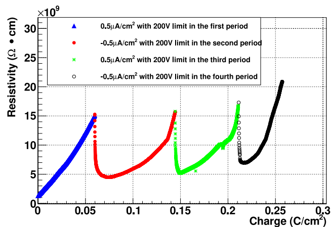
Fig. 13. Long term performance of the glass by reversing the electric field.
