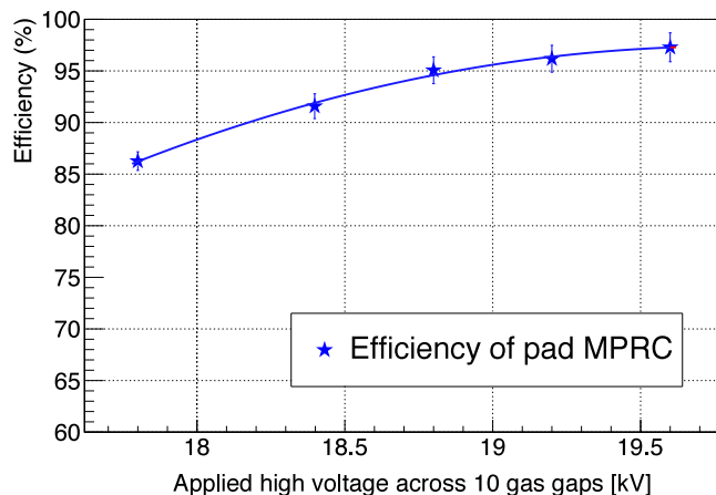
Fig. 3. The efficiency of the MRPC as a function of different voltages at 2 kHz/cm 2 . The line through the data points is to guide the eye.
