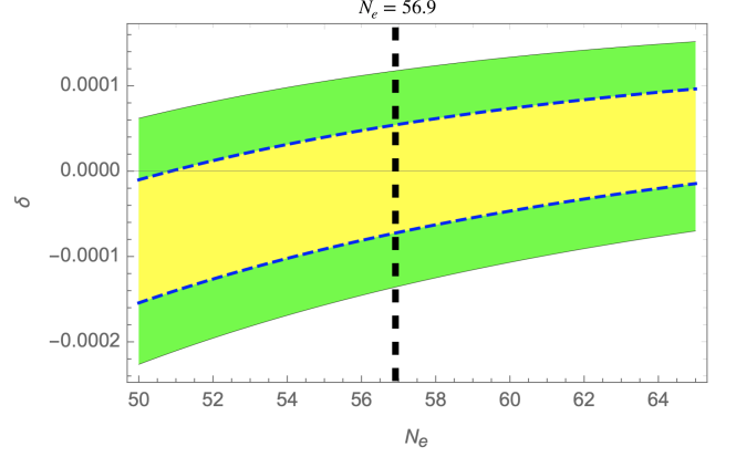
FIG. 2: The bound on \delta for varying N_e \in (50, 65) from Planck2018 1\sigma (Yellow) and 2\sigma (Green) constraints [1]. N_e = 56.9 is indicated by the vertical, dotted line.
