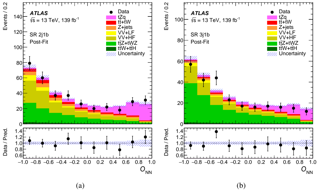
Figure 3: Comparison between data and prediction ('Pred.') after the fit to data ('Post-Fit') under the signal-plus-background hypothesis for the fitted distributions of the neural network output O_{NN} in the SRs (a) 2j1b and (b) 3j1b. The uncertainty band includes both the statistical and systematic uncertainties as obtained by the fit. The lower panels show the ratios of the data to the prediction.
