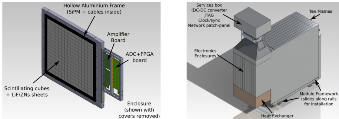
Figure 8: (Left) CAD rendering of a detector plane and its aluminium electronics enclosure. The 64 MPPCs are connected via an interface plate using twisted-pair ribbon cables that terminate into insulation displacement connectors. (Right) Diagram of a ten planes detector module with its services box and its heat exchanger, placed below to take off heat generated by the electronics [51].
