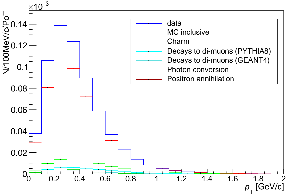
Fig. 6 Transverse momentum distributions from data and simulation, top full range in log scale, bottom detail of lower transverse momentum with a linear scale. The distributions are normalized to the number of POT. For the simulation, some individual sources are highlighted, muons from charm (green), from dimuon decays of low-mass resonances in Pythia8 (cyan), in Geant4 (turquoise), photon conversion (dark green) and positron annihilation (brown).
