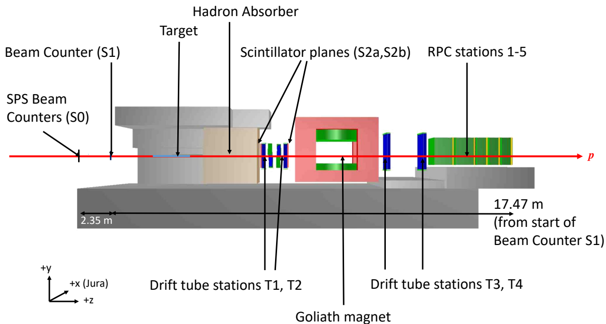
Fig. 1 Layout of the experimental setup to measure the \mu -flux. The FairShip (the SHiP software framework) coordinate system is also shown.
