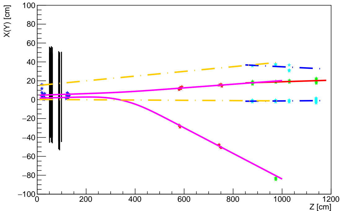
Fig. 2 A two-muon event (most events are single-muon events) in the event display. The blue crosses are hits in Drift-tube stations T1 and T2, the red crosses are hits in T3 and T4. The green and light blue are hits in the RPC stations. The orange (blue) dotted lines are drift tube (RPC) track segments in the y projection; the pink (red) curves are track segments in the x projection.
