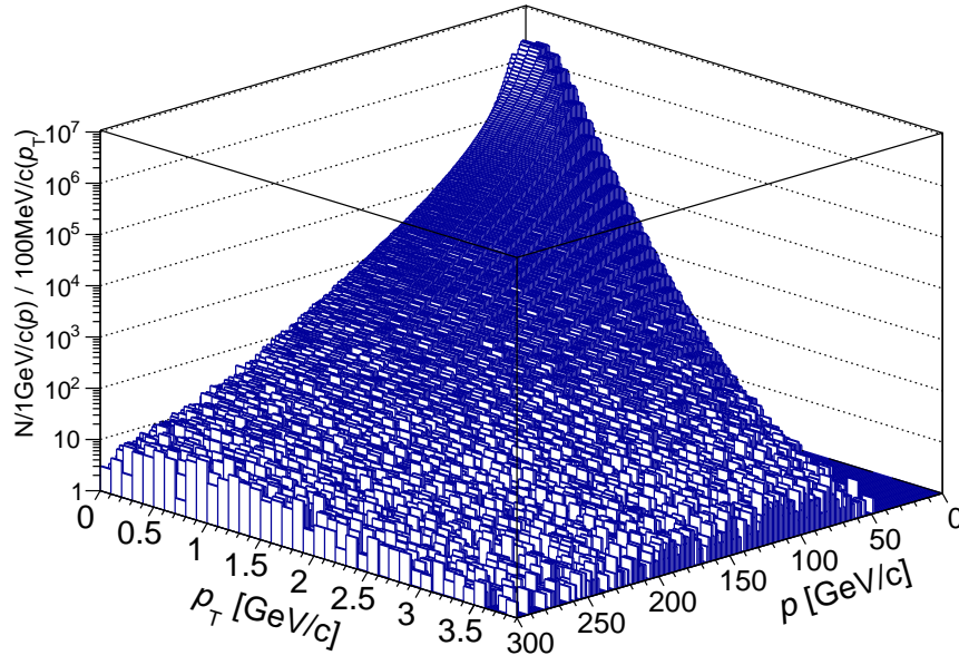
Fig. 8 p_T vs p for data. The units on the vertical axis are the number of tracks per p, p_T bin in the entire data set.
