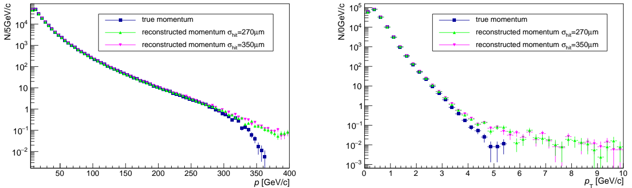
Fig. 4 Effect of additional Gaussian smearing on the momentum distribution in the simulation, left p , right p_T . The distributions correspond to the simulation truth before reconstruction (navy blue), the nominal resolution \sigma_{\text{hit}} = 270 \mu\text{m} (green) and a degraded resolution \sigma_{\text{hit}} = 350 \mu\text{m} (pink).
