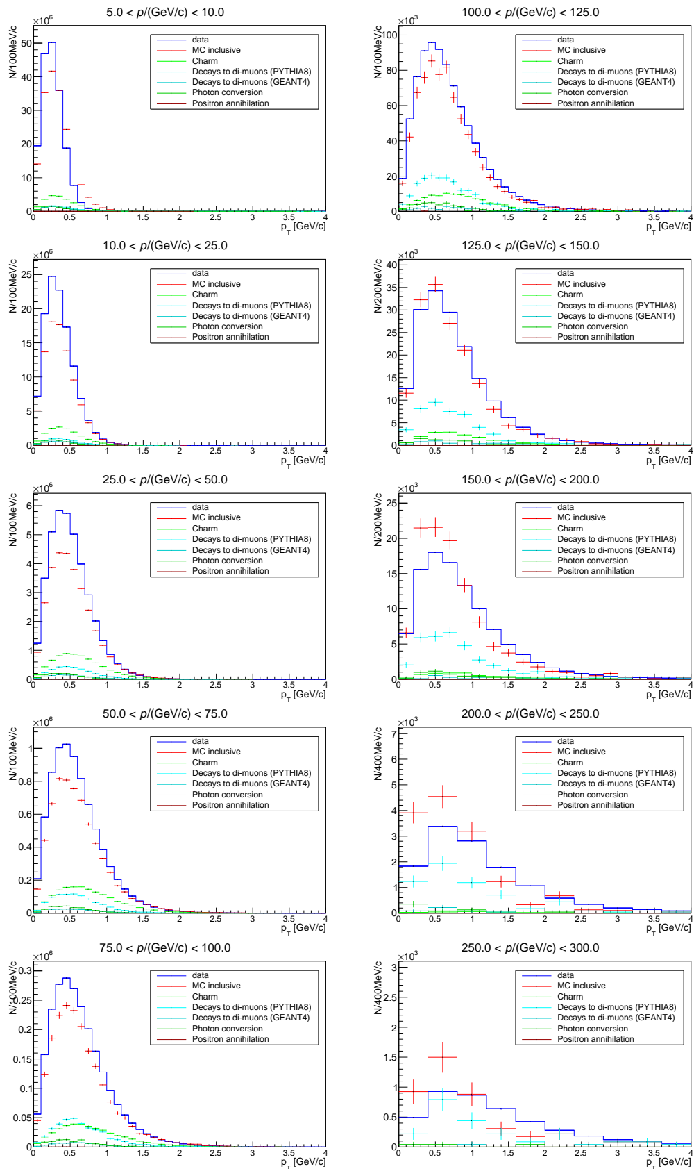
Fig. 7 p_T distributions in slices of p for data and simulation. The units on the vertical axes are the number of tracks per bin, with the simulation normalised to the data.
