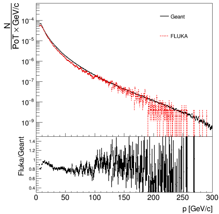
Fig. 10 Momentum distributions from FLUKA and GEANT4. The distributions are normalized to the number of POT.
