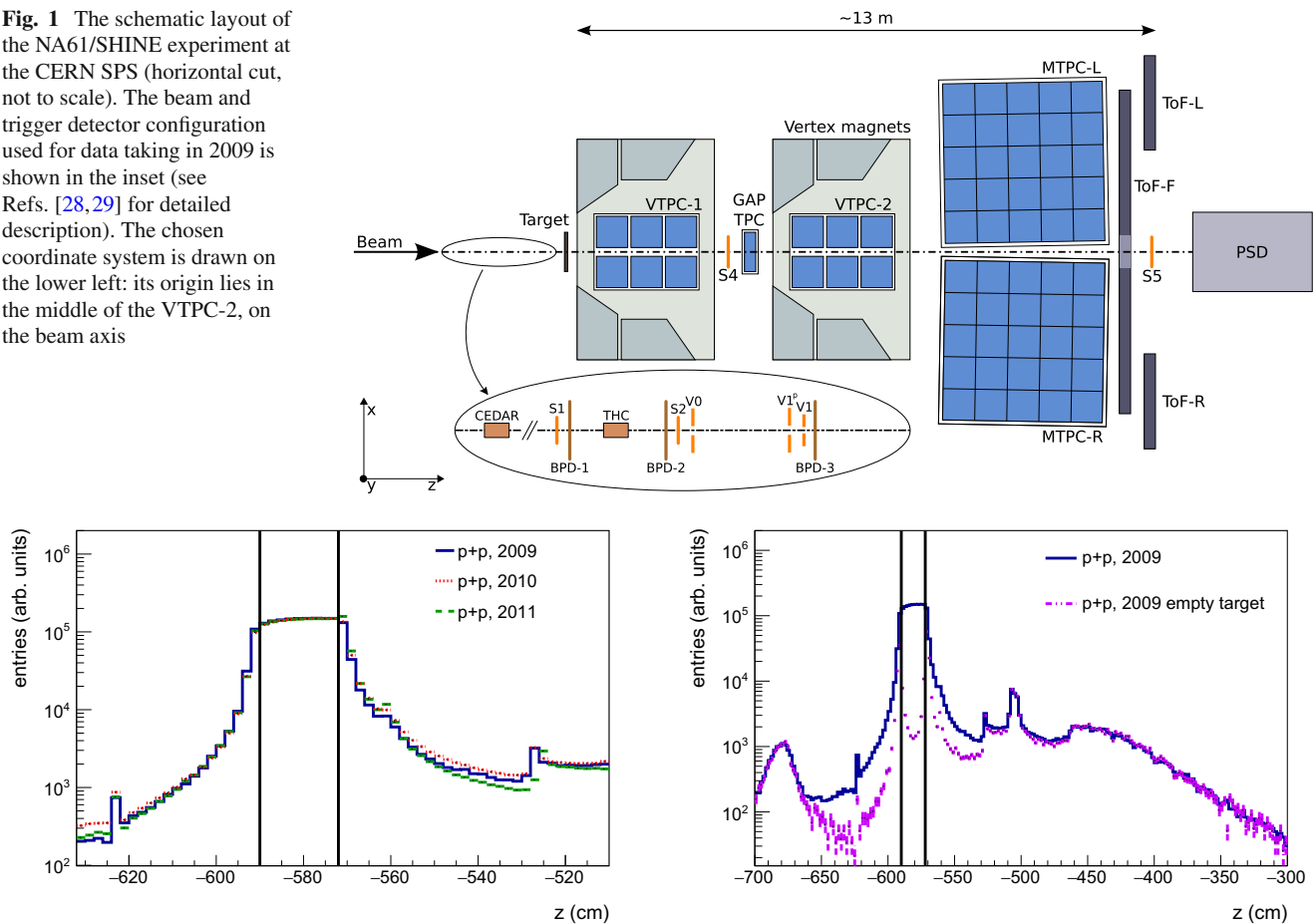
Fig. 2 Left: distributions of the z -coordinate of the reconstructed interaction vertex ( z ) for events recorded with the target inserted (2009, 2010 and 2011 data). Histograms are normalized to the same integral in the range -590 < z < -572 cm. Right: distributions of the z -coordinate of the reconstructed interaction vertex for target-inserted
